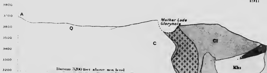
Structural section A-A' Scale, horizontal and vertical.
