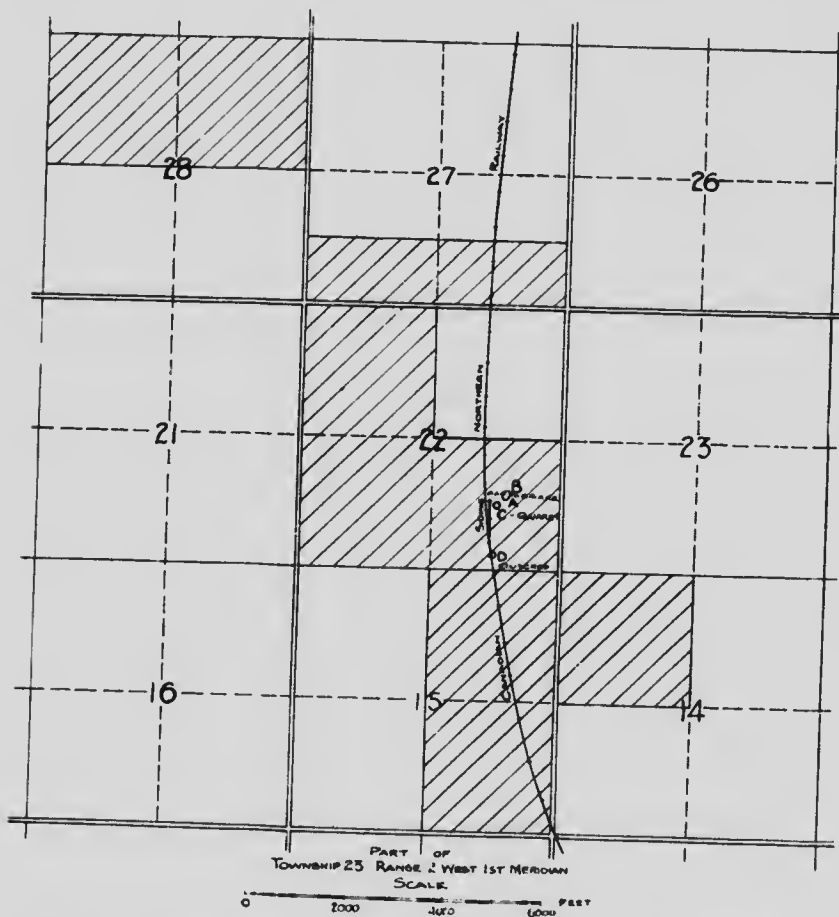
Fig. 5. Plan of the property of the Manitoba Stone Works, Broadvalley, Man.
