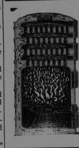
THE MOST PERFECT HOT WATER HEATING BY GURNEY'S BOILER & NEW RADIATOR.
