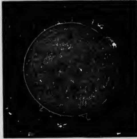
The Sun
