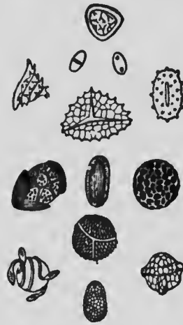
Spores
