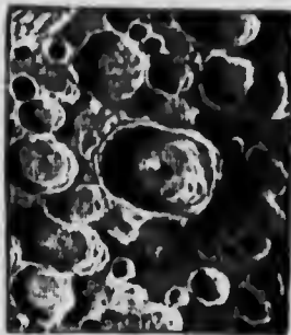
A part of the moon's surface
