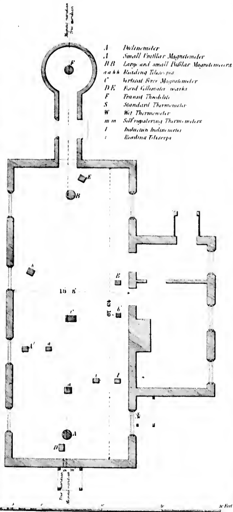
Plan of the Toronto Observatory showing the Disposition of the Instruments
