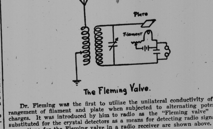
The Fleming Valve.
