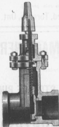
Sluice Valve
