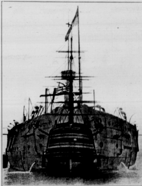
THE LARGEST WARSHIP AFLOAT AND THE OLDEST WARSHIP IN COMMISSION The above most interesting picture, which is composite, illustrates one of the many remarkable developments in warship building which have taken place between 1755 and 1911. It shows the beams of the Hercules and Nelson's flagship the Victory. A photograph of each vessel was made, with the camera at a fixed distance. Then the two negatives were printed on the same piece of photographic paper. The Victory, it will be noted, could be easily stowed away in the Hercules.
