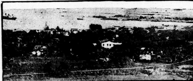
View of the City of Hilo, Hawaii, near which Kilauea is located.
