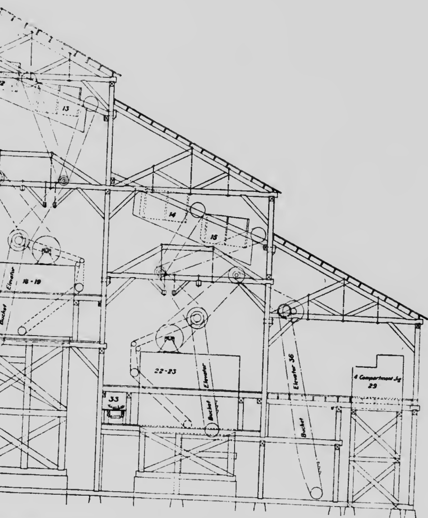
Processing plant at Austin Brook. The Canada Iron Corporation, Limited.
