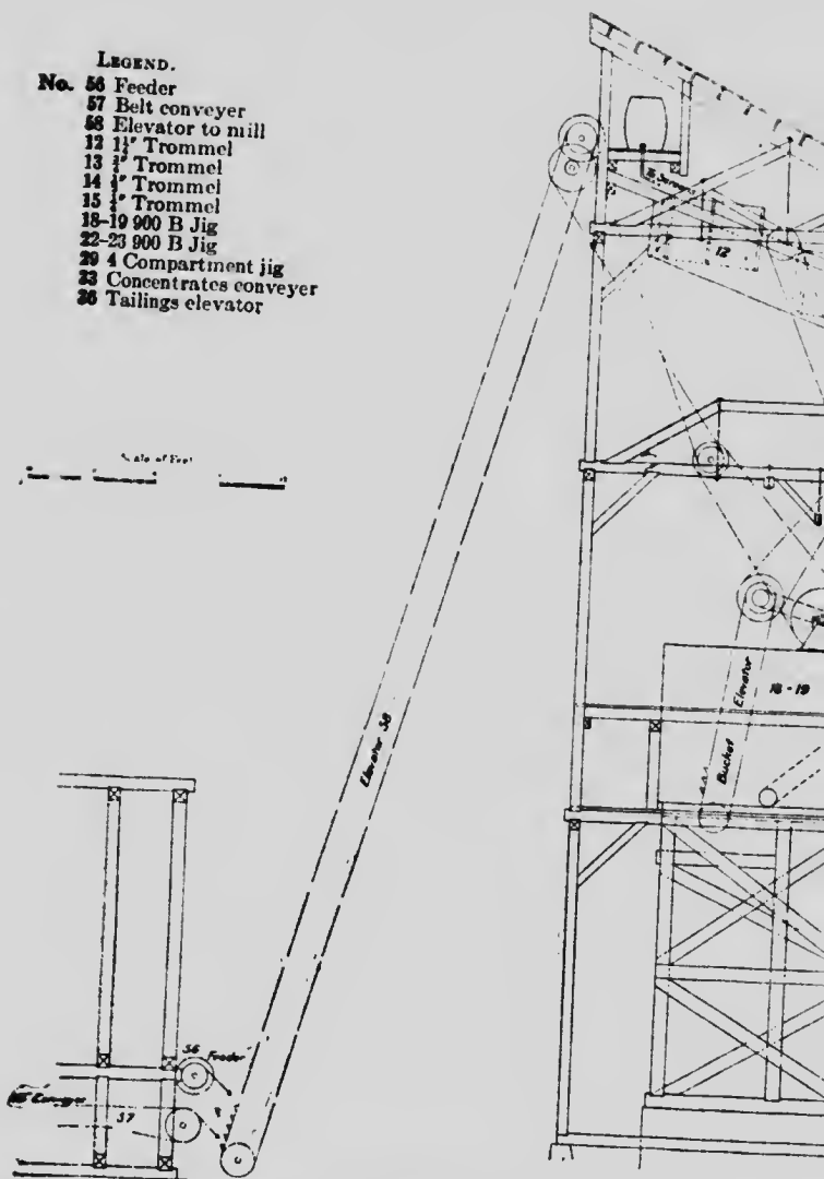
FIG. 5. Section between 3 and 4 (Fig. 4) of concentrating plant
