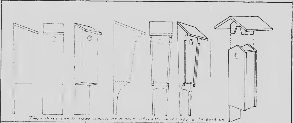
These boxes can be made wholly or in part of waste mill sabs, with a dash on
