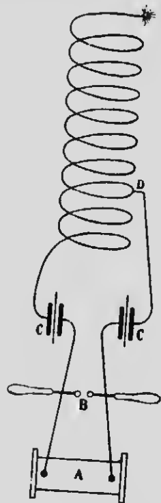
FIG. 128.—PLAN OF OUDIN'S RESONATOR.
