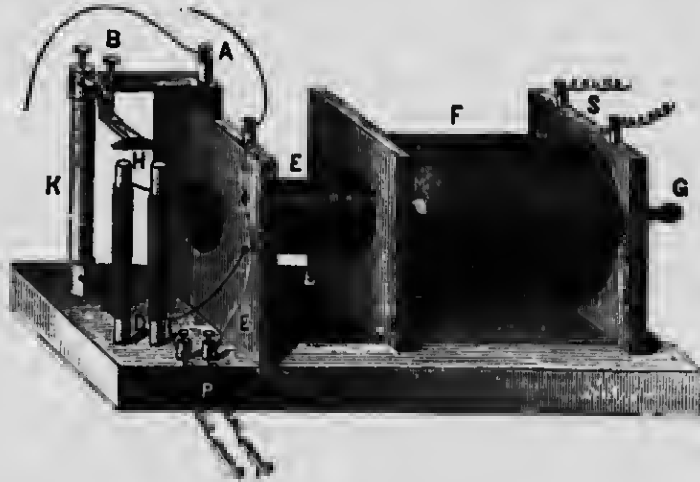
FIG. 17.—INDUCTION COIL.
