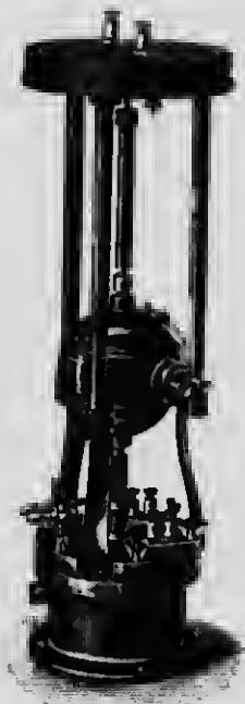
FIG. 114.—MERCURY INTERRUPTER FITTED WITH MICA DISC RECTIFIER.
