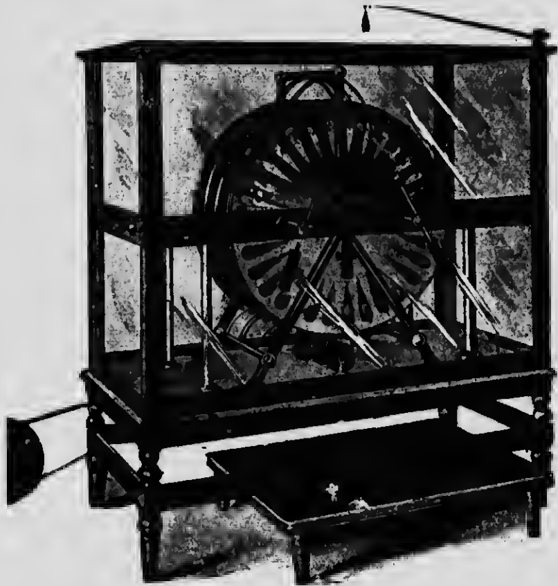
FIG. 118.—WIMSHURST MACHINE.
