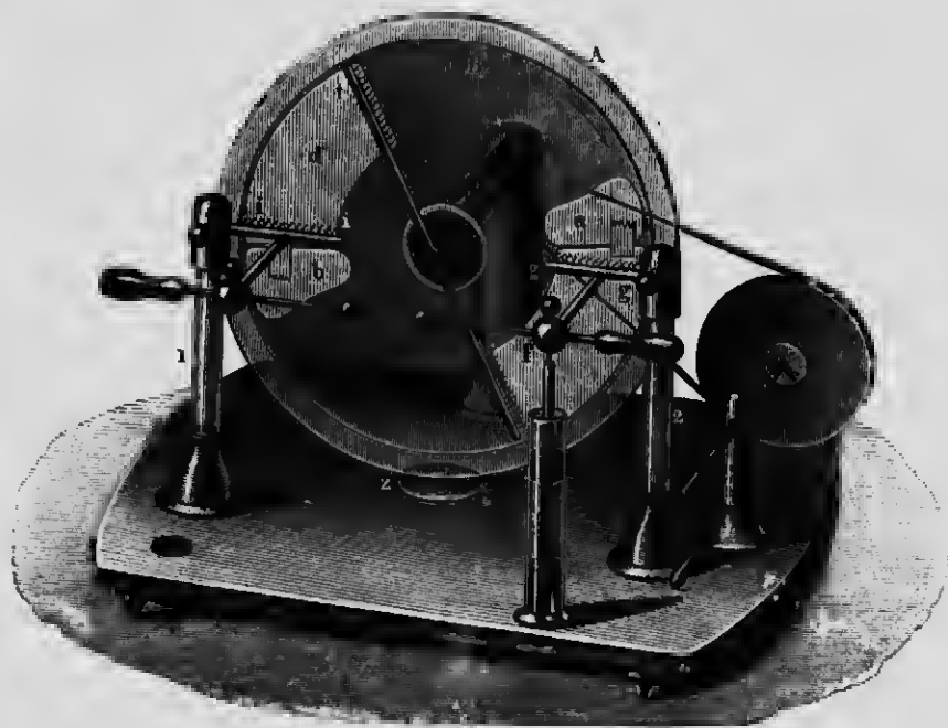
FIG. 115.—HOLTZ MACHINE.
