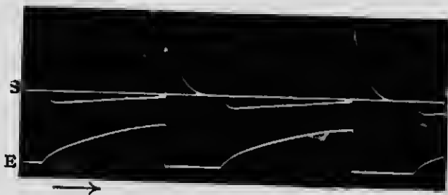
FIG. 35.—CURRENT CURVES OF COIL WITH LONG WINDINGS, AND WITH IRON CORE S, secondary curve ; E, exciting current.
