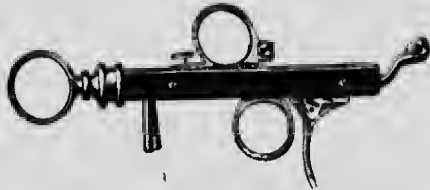
FIG. 61.—SCHECH'S CAUTERY HOLDER.
