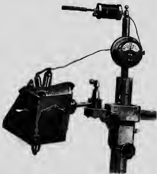
FIG. 149.—DETAILS OF TUBE-STAND, SHOWING MILLIAMPEREMETER AND ENCLOSED SPARK-GAP RECTIFIER ATTACHED TO IT.
