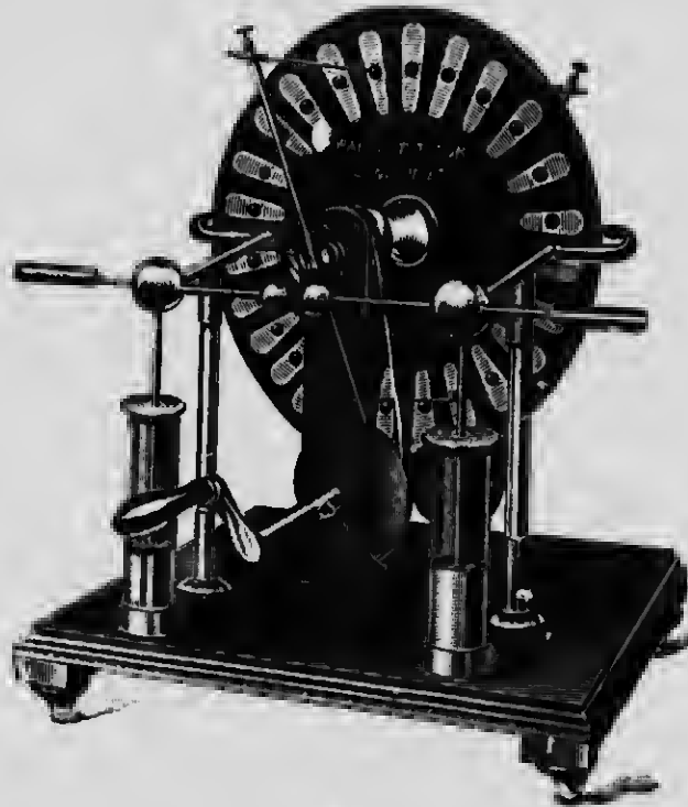
FIG. 117.—WIMSHURST MACHINE.
