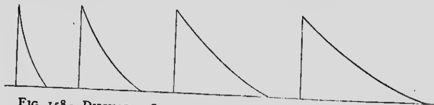
FIG. 158.—DISCHARGE CURVES OF CONDENSERS WHEN THEIR CAPACITIES ARE IN THE RATIOS OF 1, 2, 3, 4, WITH CONSTANT VOLTAGE AND CONSTANT RESISTANCE.
