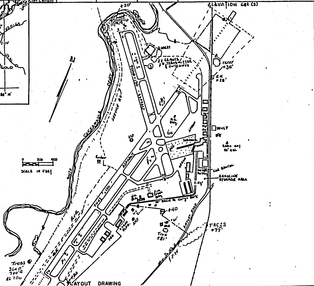
LAYOUT DRAWING
