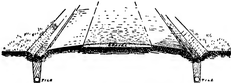
Fig. 83.—A gravel road properly crowned, with side ditches and tile drains.
