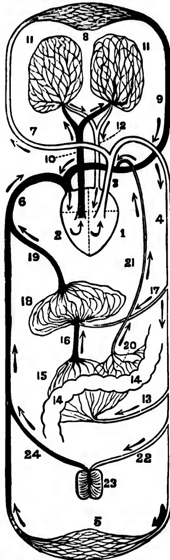
Fig. 80.—The circulation of the blood in the body.
