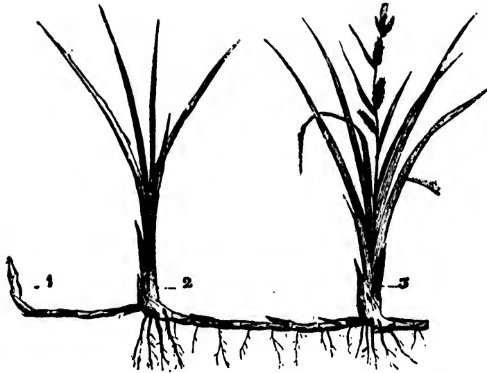
Fig. 22.—Illustration showing how some plants reproduce by creeping roots. 1, new plant just coming up; 2, plant before blossoming; 3, old plant forming seed. June grass and couch grass spread in this way.
