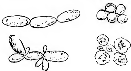
Fig. 79.—Yeast plant, magnified.
