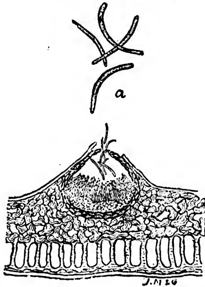
Fig. 65.—Section of a diseased plum leaf, spores being thrown off. a Spores very much enlarged. See Figs. 42 and 43.
