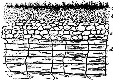
Fig. 18—Soil formed from rock underneath. a soil with grass growing in it; b subsoil, coarser and more rocky; c coarse, loose rock; d rock in layers, cracked. d changes to c , c changes to b , and b to a .
