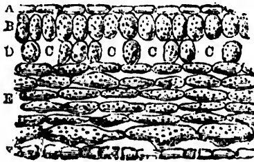
Fig. 12.—Section of a Leaf. A , row of cells forming skin on upper side; B , row of cells next to skin; D , next row of cells; C , air spaces in leaf; E , inner portion of cells filled with sap; F , row of cells forming under skin of leaf showing mouths or openings (stomata).
