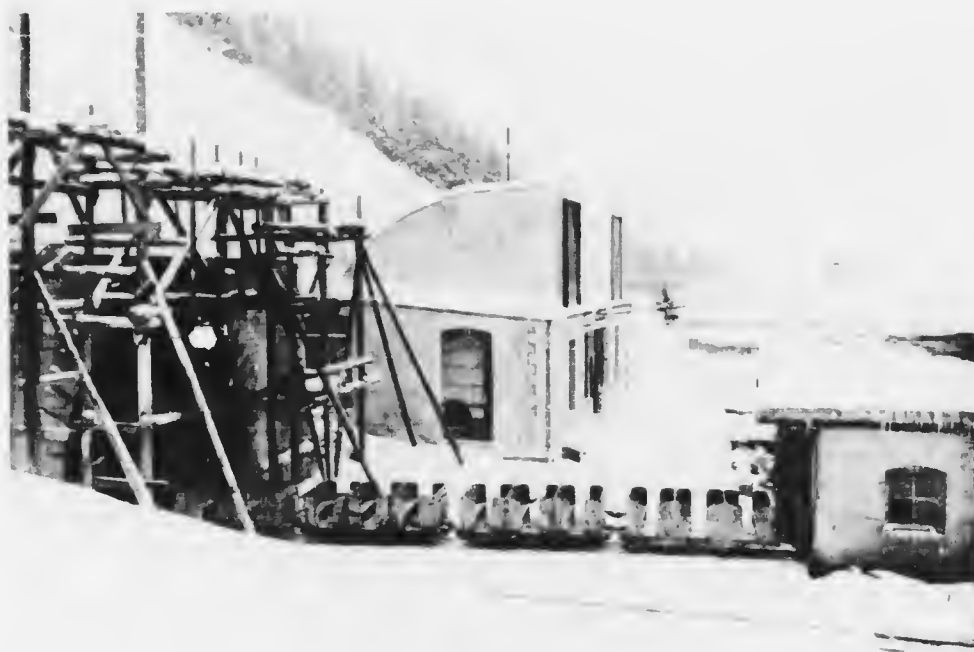
THE NORTHERN ENTRANCE TO THE LOTSCHBERG TUNNEL AT KANDERSTEG. Showing workmen's train and ventilating pumping-station.
