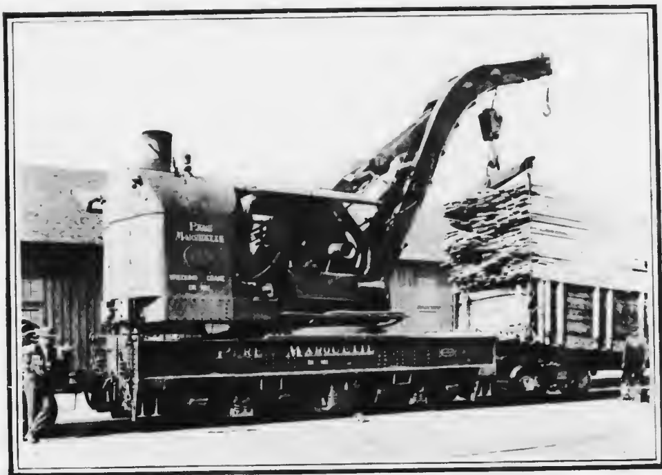
AN INDUSTRIAL WORKS' BREAKDOWN CRANE LIFTING A WAGON BODY AND ITS LOAD TO AFFORD ACCESS TO THE WHEEL TRUCK.
