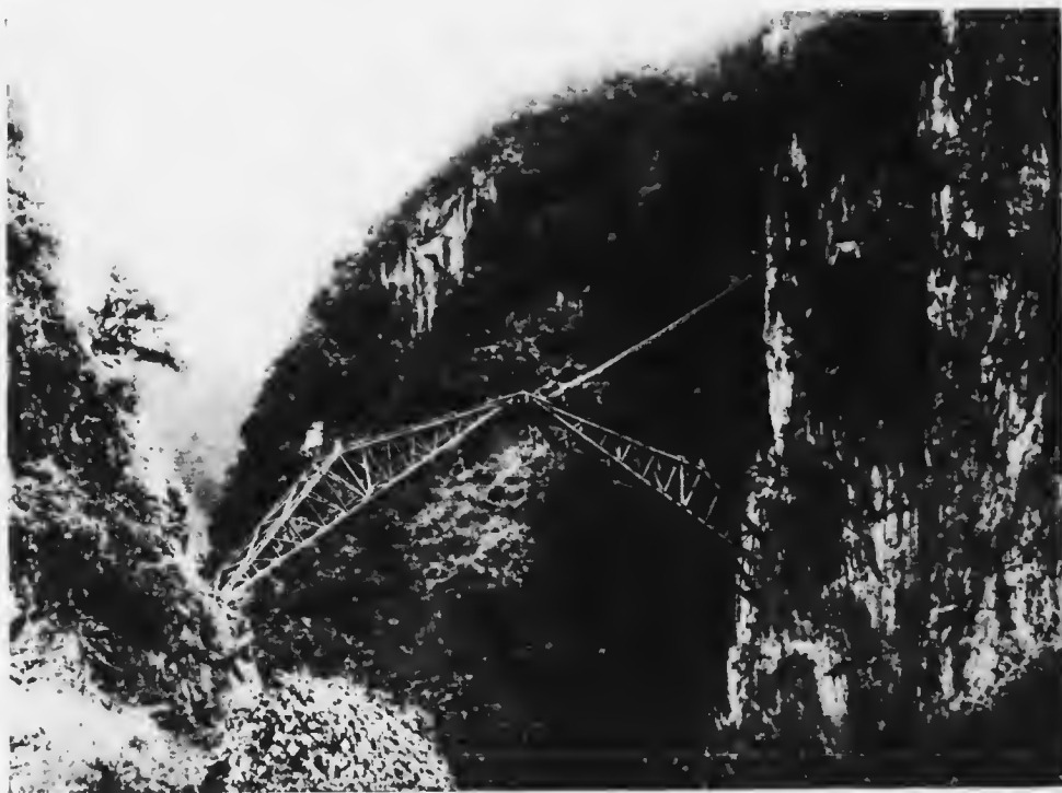
THE BASCULES OF THE FAUX NAM-TI BRIDGE SET AND CONNECTED. Showing the ropes whereby each section was lowered.
