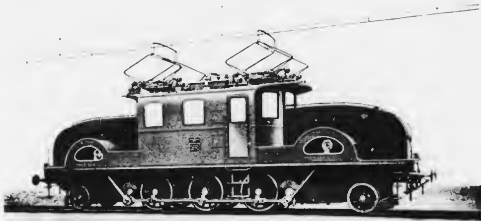
THE 2-6-2 ELECTRIC LOCOMOTIVE USED ON THE PRUSSIAN STATE RAILWAYS.
