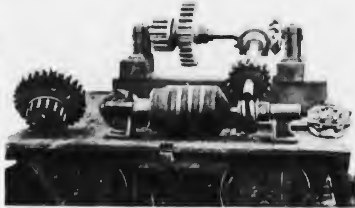
THE GEAR OF EDISON'S FIRST ELECTRIC LOCOMOTIVE.
