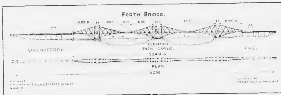
PLAN AND ELEVATION OF THE BRIDGE
