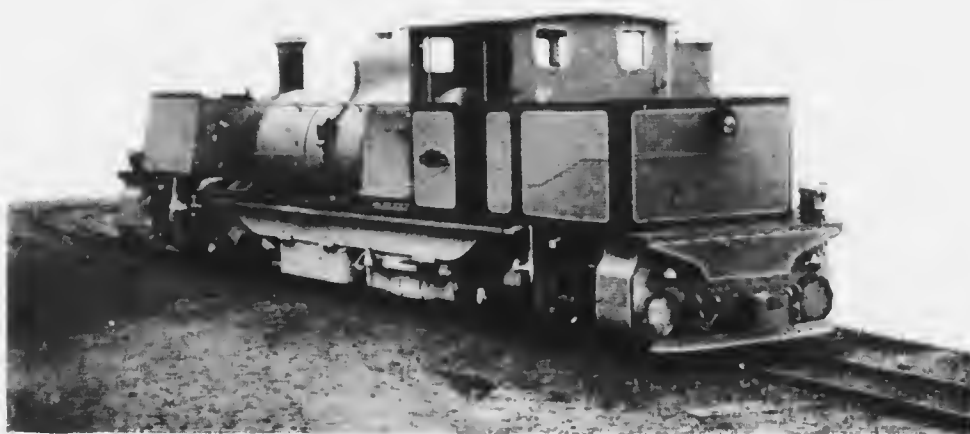
A GARRATT LOCOMOTIVE FOR THE DARJEELING-DIMALAYAN RAILWAY, ON A REVERSE CURVE OF 60 FEET RADIUS.
