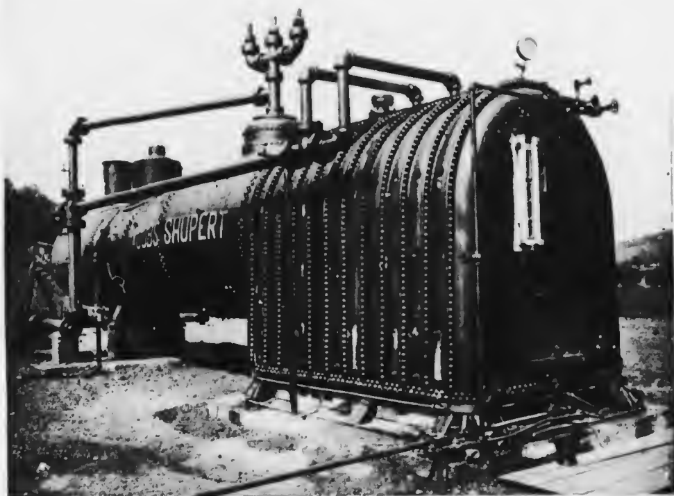
EXTERIOR VIEW OF BOILER, WITH JACOBS-SHUPERT FIRE-BOX, IMMEDIATELY AFTER LOW WATER TESTS
