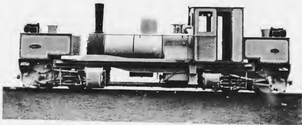
1111 GARRATT PATENT LOCOMOTIVE, USED ON THE TASMANIAN GOVERNMENT RAILWAYS NORTH-EAST DUNDAS SECTION.
