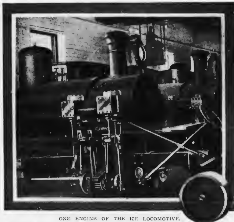
ONE ENGINE OF THE ICE LOCOMOTIVE.
