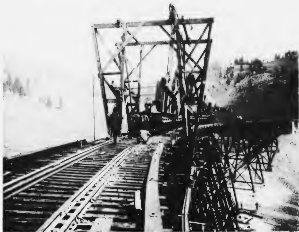
REBUILDING IN STEEL THE OLD TIMBER TRESTLE ACROSS GREENHORN GULCH IN THE ROCKY MOUNTAINS.
