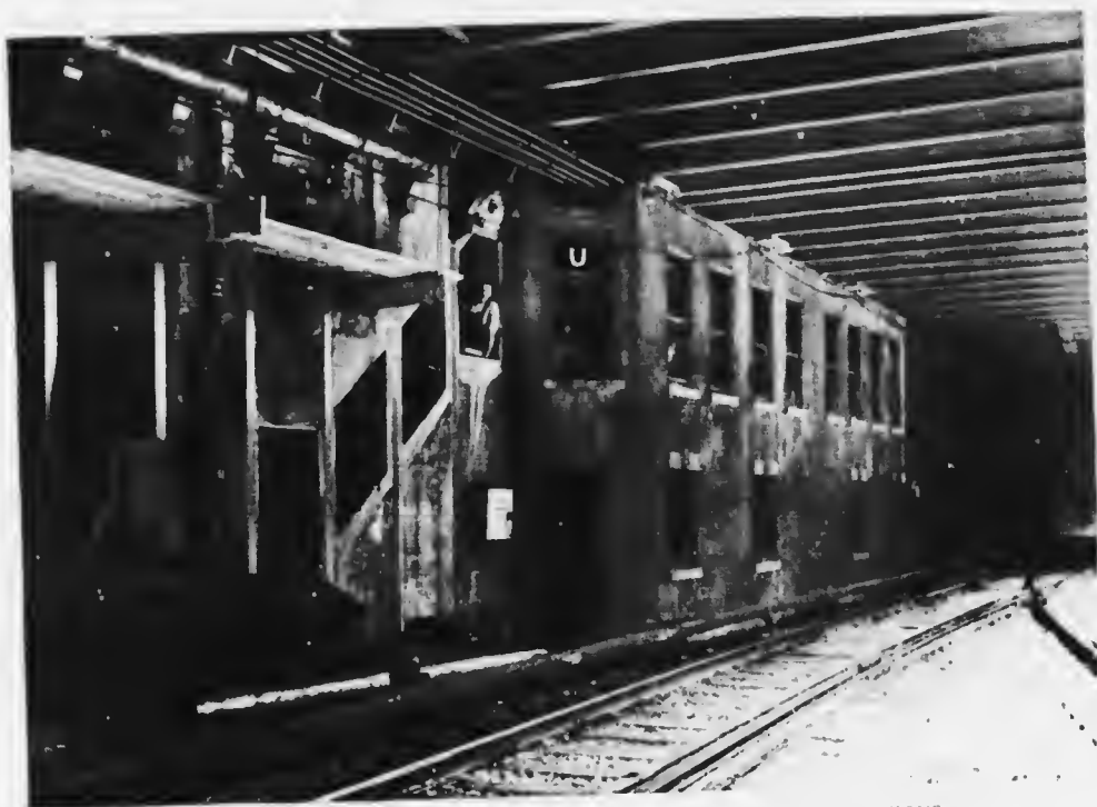
EXTERIOR OF ONE OF THE UNDERGROUND INTERLOCKING STATIONS Above this cabin on the street level is a 12-floor skyscraper.
