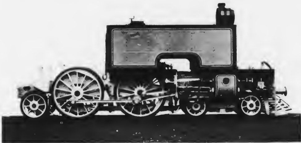
Front Engine Unit.
