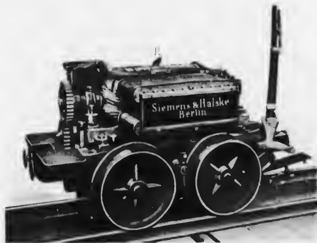
Reproduced by Messrs. Siemens Brothers & Co., Ltd. THE 3-HORSE-POWER ELECTRIC LOCOMOTIVE INVENTED BY WERNER VON SIEMENS IN 1879
