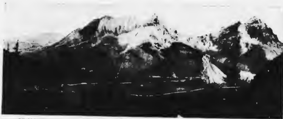
RE-ALIGNMENT OF THE CANADIAN PACIFIC RAILWAY THROUGH KICKING HORSE PASS. View showing the amazing location of the new line and spiral trestles. The old line runs through the centre. The new line doubled the distance (8.2 miles), but halved the grade (2.2 per cent.—116 ft. per mile).
