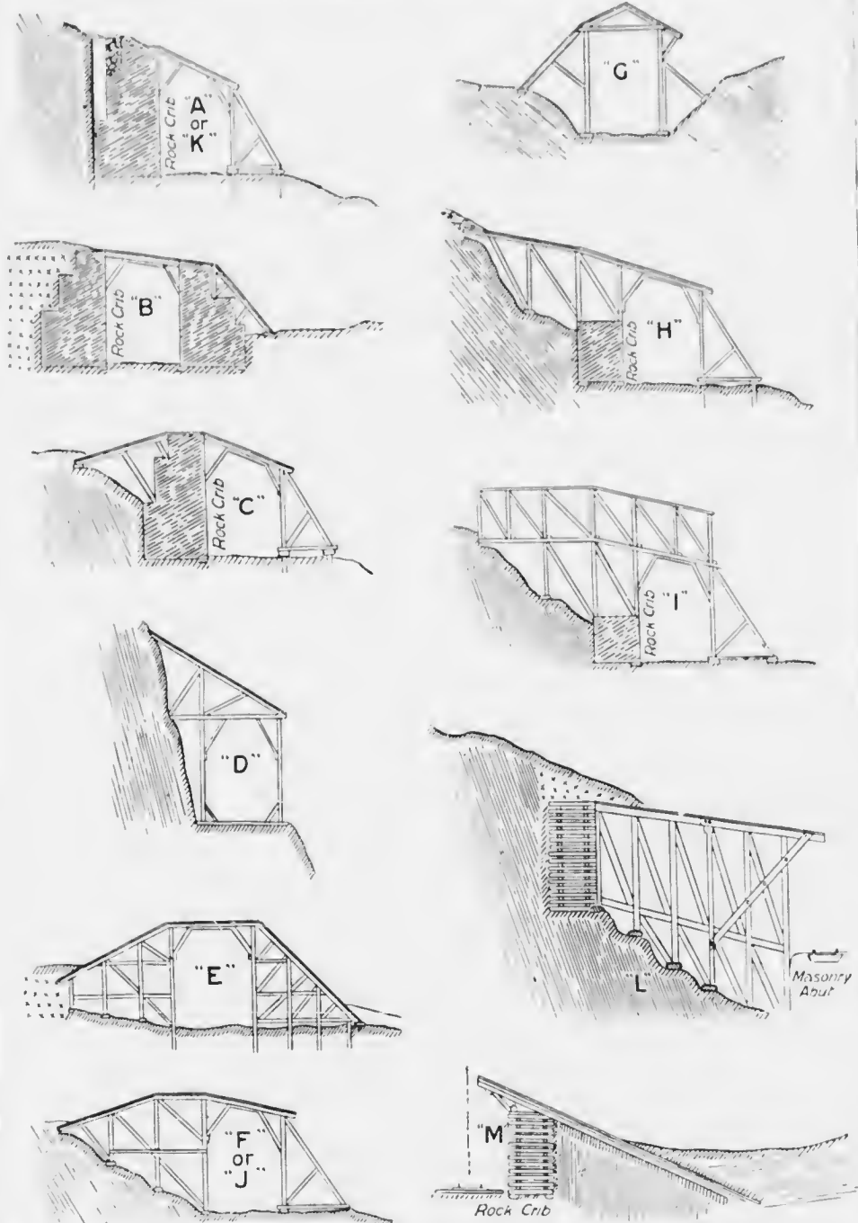
DIFFERENT TYPES OF SNOW-SHEDS.
