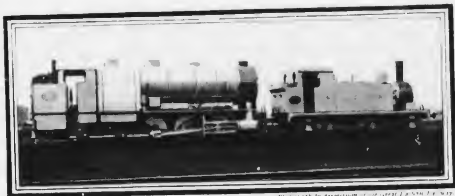
THE GREAT EASTERN "DECAPOD" IN COMPARISON WITH AN ORDINARY TANK ENGINE.
