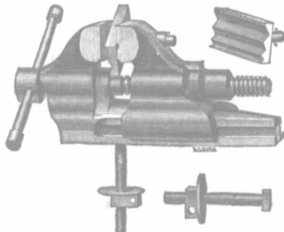
PIPE-EXTRA JAW.
