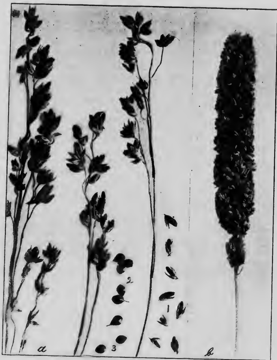
Plate 7. (a) Smut of broom corn (1) smut balls; (2) normal parts of ear enclosing sound grain; (3) sound grain of broom corn (b) An ear of millet affected with smut.
