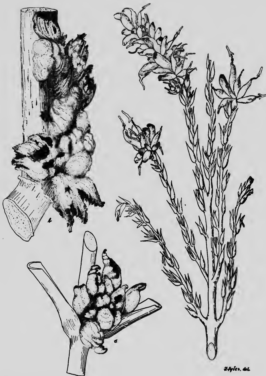
Plate 6. Smut of corn. (a) Male inflorescence partly infected. (b) A large "smut boil" on the main stem. (c) Female inflorescence or "cob" destroyed by smut.
