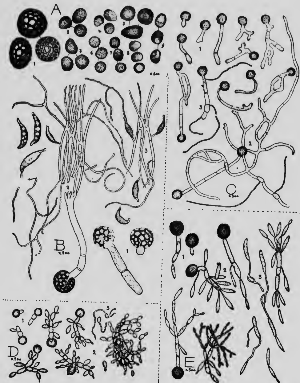
Plate 9. A 1-9 three spores of each kind of smut treated in this bulletin, all magnified 600 times. (1) Stinking smut of wheat, (2) naked smut of oats, (3) smut of millet, (4) loose smut of wheat, (5) corn smut, (6) broom corn smut, (7) loose smut of barley, (8) covered smut of barley, (9) covered smut of oats. B. Germination of stinking smut spores. (1) Early stages showing bursting of spore wall and promycelium growing. (2) Stout promycelium tube terminates in a crown of points at which the wreath of secondary sickle-shaped spores is produced, some of which are shown germinating. (3) Secondary spores producing tertiary spores and 4 tertiary spores enlarged, one germinating into infection tube. C. Germination of loose smut spores of wheat, (1) early stages, (2) a spore observed in artificial cultures for 12 days, (3) the promycelium produces thin infection tubes. D. Naked smut spores of oats germinating. (1) Early stages, (2) showing masses of secondary spores produced, (3) two secondary spores producing infection tubes. E. Corn smut spores germinating. (1) Early stages, (2) production of secondary spores, (3) secondary spores germinating, (4) production of air conidia from secondary conidia.
