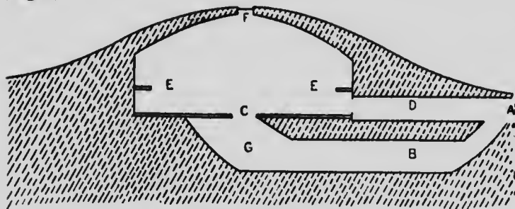
Fig. 1. Side elevation of St. Michael Kázgi .
