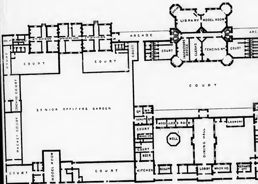
GROUND PLAN OF THE WHOLE.
