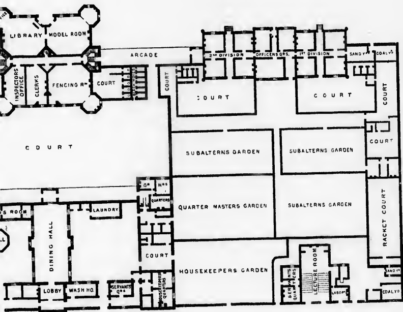
GROUND PLAN OF THE WHOLE.
