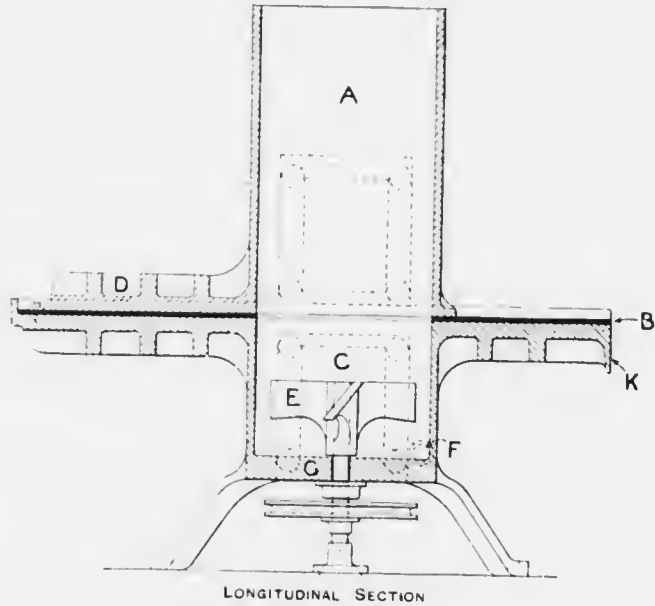
FIG. 66. THE SLIDE MACHINE.
