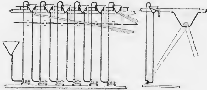
FIG. 22. A NEST OF CENTRIFUGAL PUMPS.
