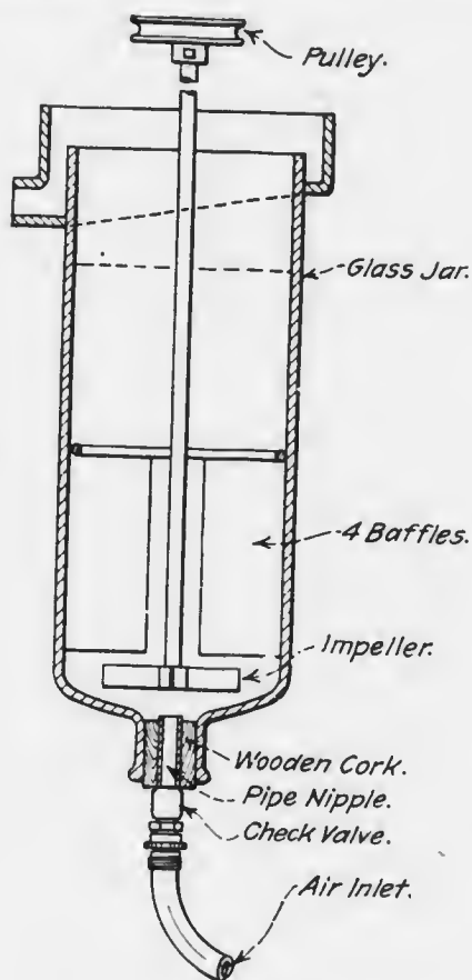
FIG. 69. OWEN TEST-MACHINE.
