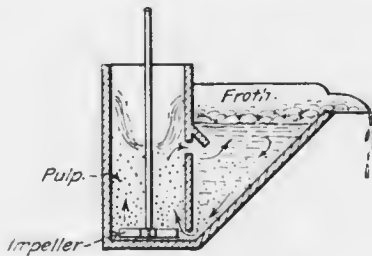
FIG. 62. ANOTHER FORM OF HOOVER MACHINE.
