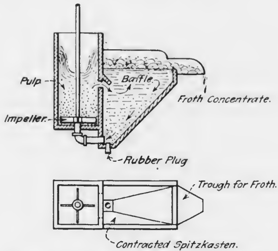
FIG. 61. SKETCH OF THE LYSTER OR HOOVER MACHINE.
