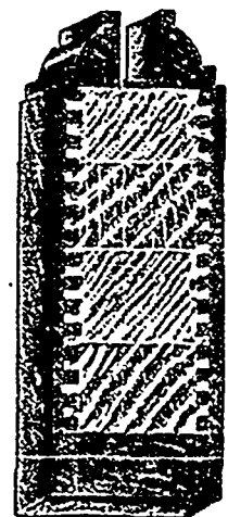
STILE SECTION
