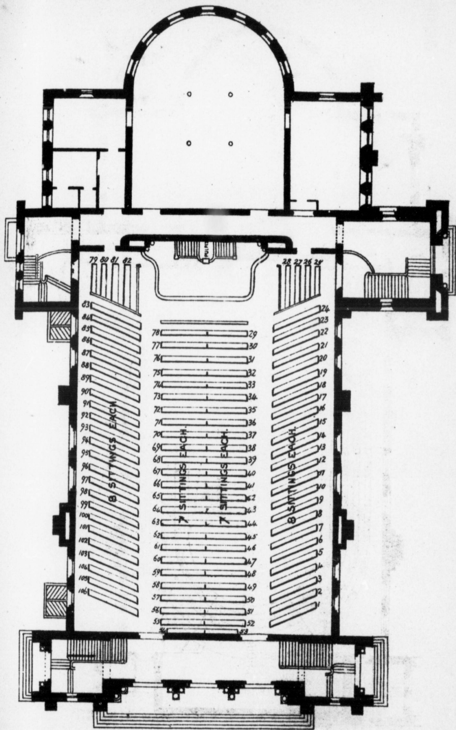
ST ANDREW'S CHURCH. PLAN OF AREA.
