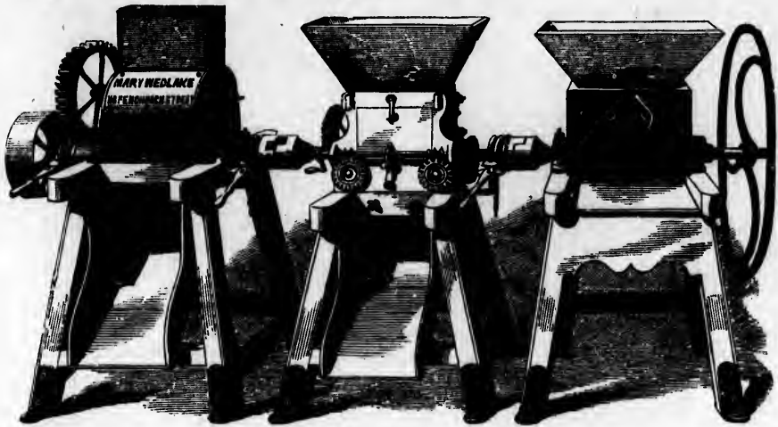
Wedlake's Union Mill for Splitting and Bruising Seeds.
