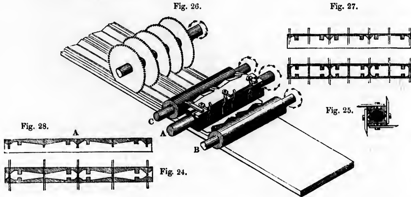
Sash-bar machine used for the building.
