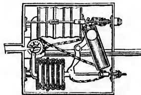
Brown's Patent Meter.
