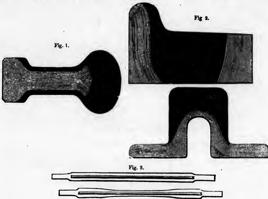
Thornycroft's Patent Axles.
