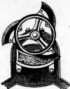
Mr. J. Smith's Patent Chaff-cutter.
