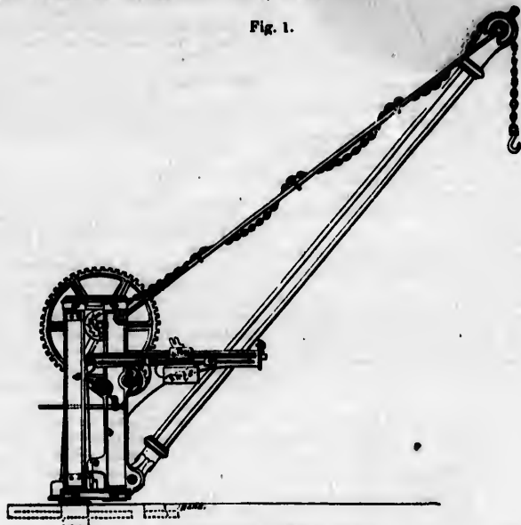
James & Co.'s Patent Weighing Crane.
