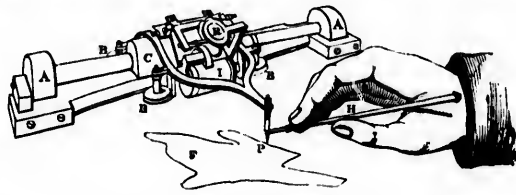
Sang's Planometer.
