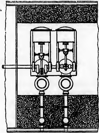
Side Elevation.
