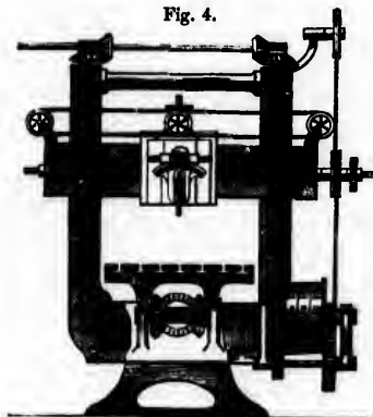
Whitworth's Self-acting Planing Machine.
