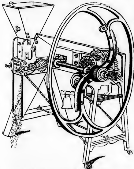
Wedlake's Chaff-cutting and Oat-bruising Machine.
