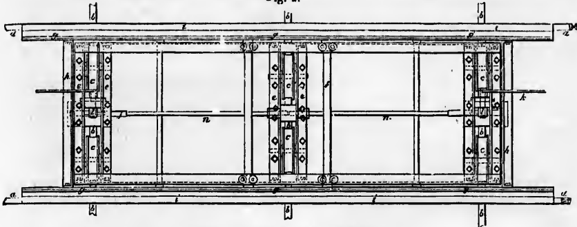
Ormerod and Son's Patent Traversing Machine.
