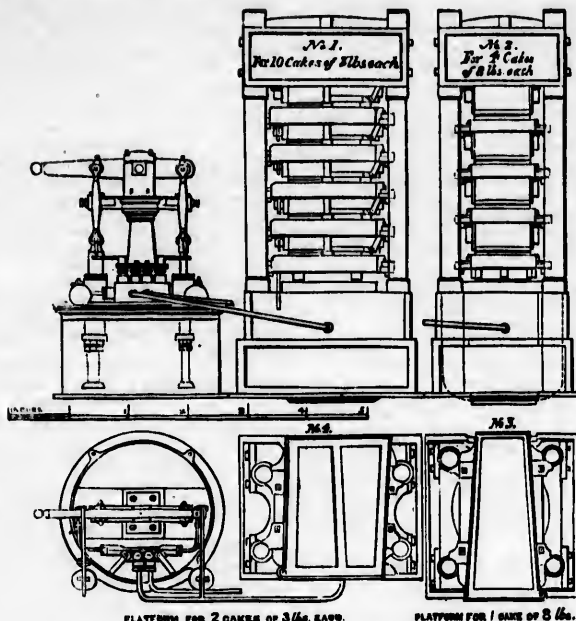
Blundel, Spence, and Co.'s Hydraulic Seed Presses.
