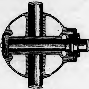
Section of Globular Nave.
