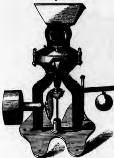
Crosskill's Mill for Vegetable Substances.
