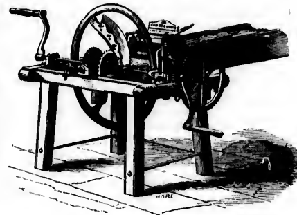
Cornes' Registered Chaff-cutting Machine.
