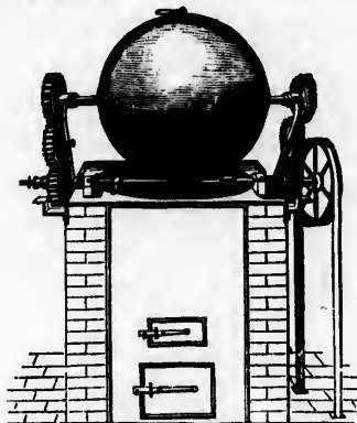
Law's Globe-roaster for Coffee.
