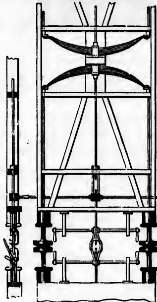
Thornton's Patent Coupling for railway Waggons.
