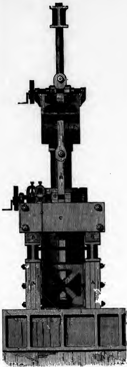
II. THE PRESS SHOWN IN OPERATION—THE TUBE PARTLY LIFTED.
