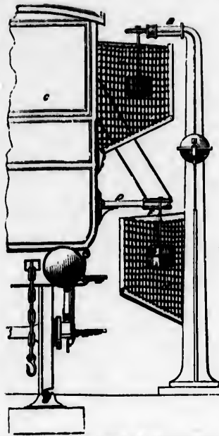
Dicker's Automatic Apparatus for Mail Trains.
