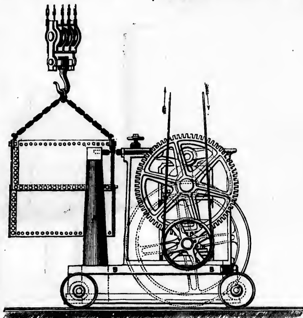
Fairbairn's Patent Riveting Machine. Side Elevation.
