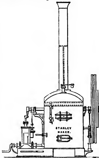
Stanley's Two-horse Portable Steam-engine. (End Elevation.)
