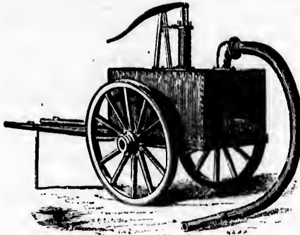
Deane and Co.'s Patent Tank-cleaner.
