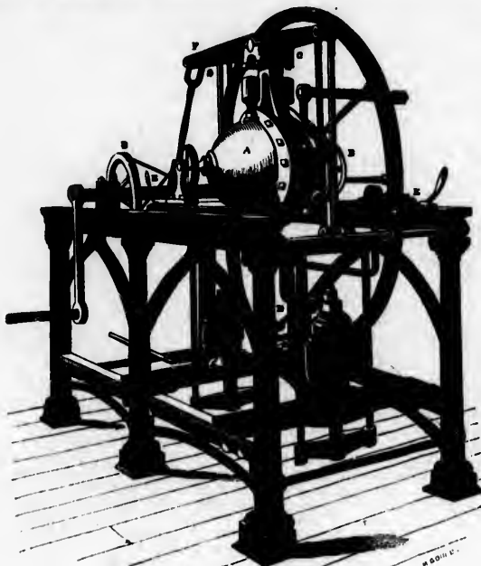
Tyler, Hayward, and Co.'s Soda-water Machine.
