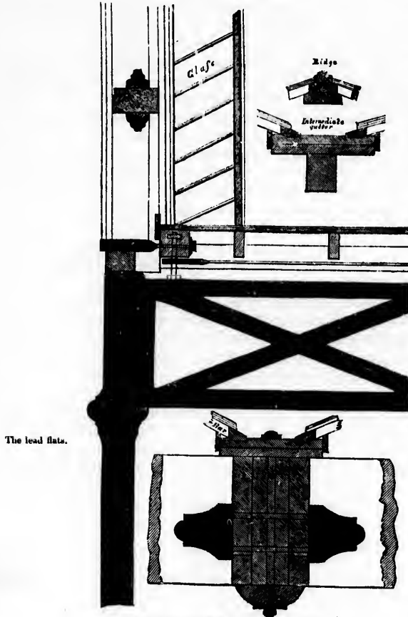
Section of Transsept Rib, and springing of ditto.
