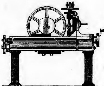
Whitworth's Self-acting Wheel-cutting and Dividing Machine.
