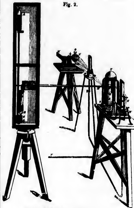
Brooke's Self-registering Barometer.
