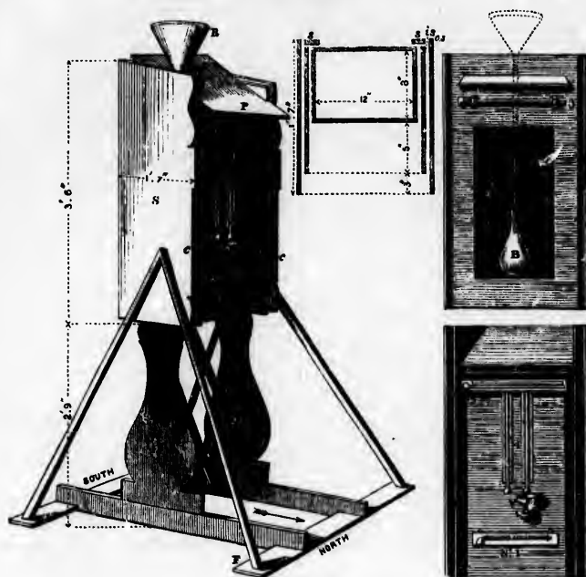
Lawson's Thermometer Stand
