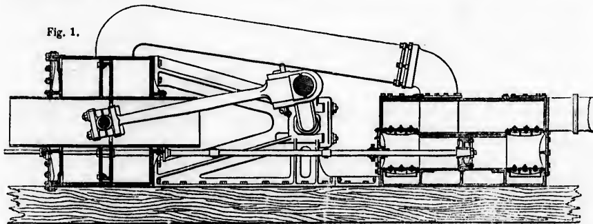
Penn & Son's Patent Marine Trunk Engines.
