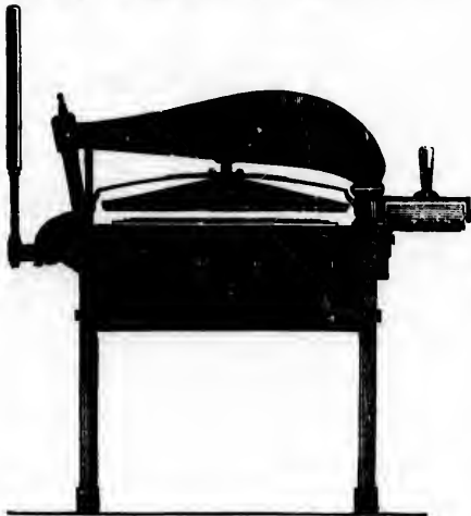
Harrild's Galley Press.
