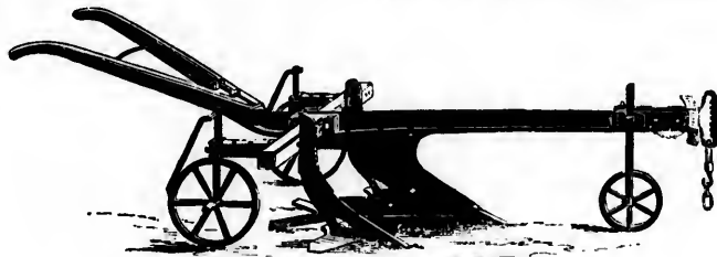
Bentall's Patent Broad Share and Subsoil Plough.
