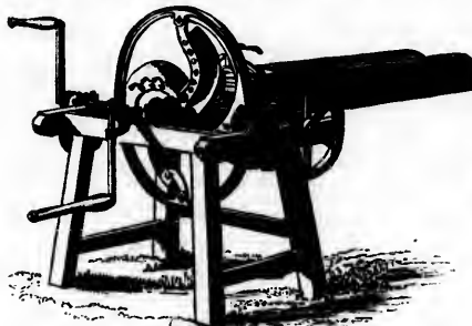
Williams' Chaff-engine.
