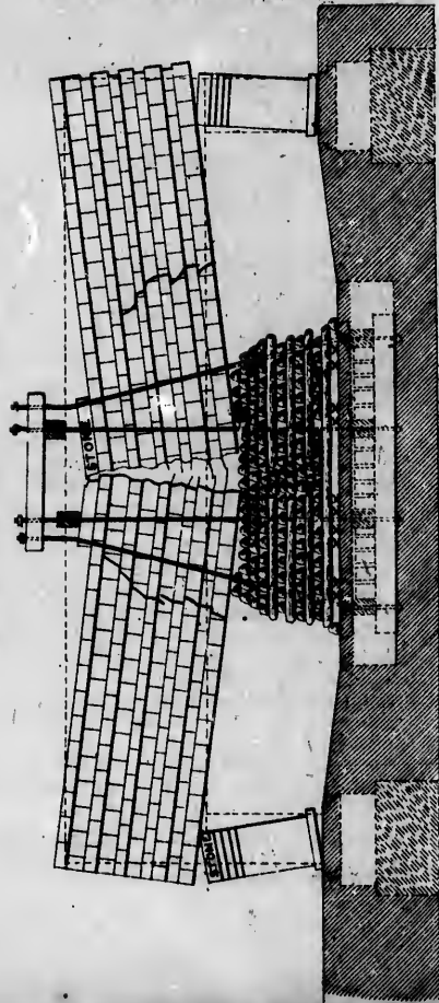
APPEARANCE OF THE BEAM WHEN BROKEN DOWN.
