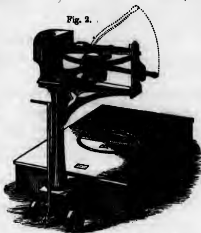
James & Co.'s Small Patent Weighing Machine.
