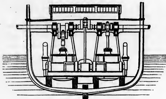
End Elevation.
