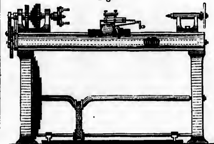
Whitworth's Self-acting Foot Lathe.
