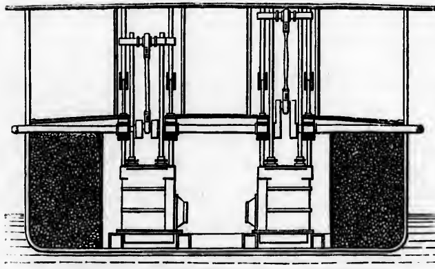
End Elevation.
