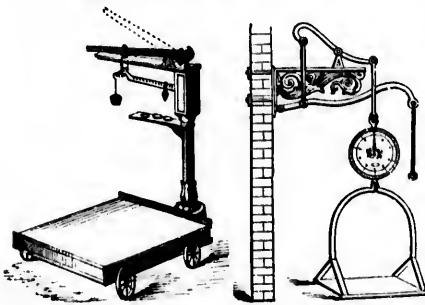
Improved Lever Weighing Machine.
