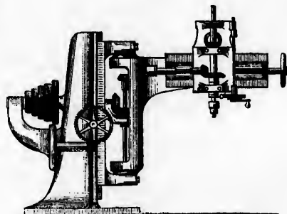
Whitworth's Self-acting Radial Drilling and Boring Machine.
