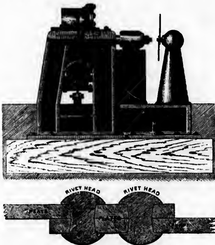
Garforth's Steam Riveting Machine.
