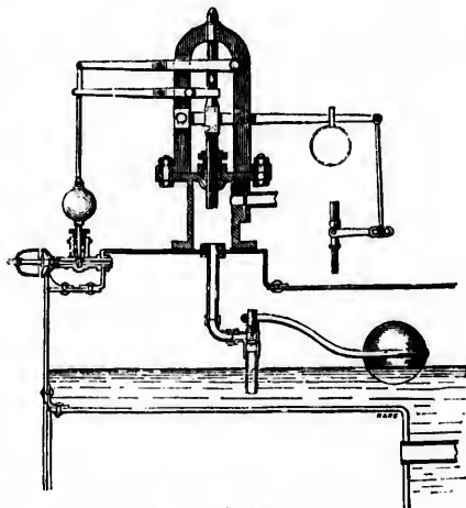
Turner's Steam-boiler Feeding Apparatus.
