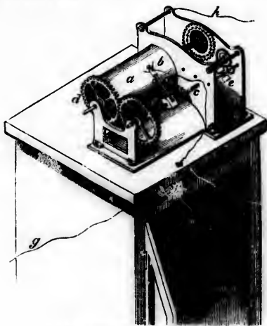
Bakewell's Copying Electric Telegraph.
