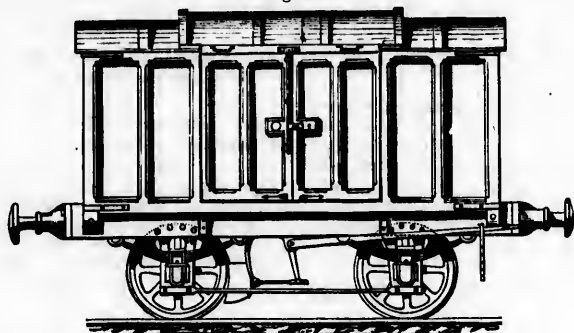
Henson's Covered Wagon. Side Elevation.
