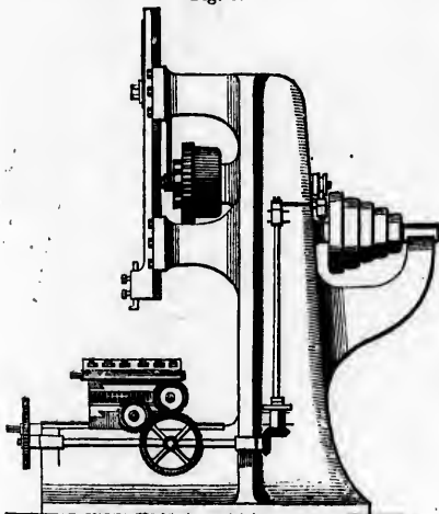
Whitworth's Patent Self-acting Slotting and Shaping Machine.
