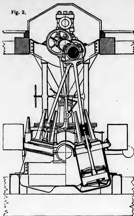
Penn &amp; Son's Marine Oscillating Engines.
