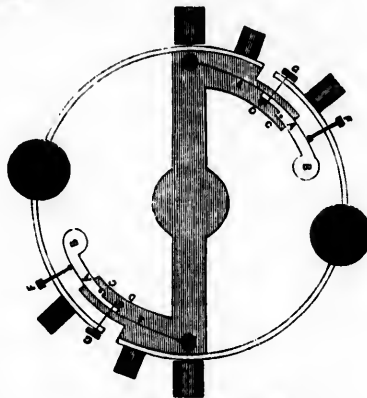
Pennington's Compensated Balance.
