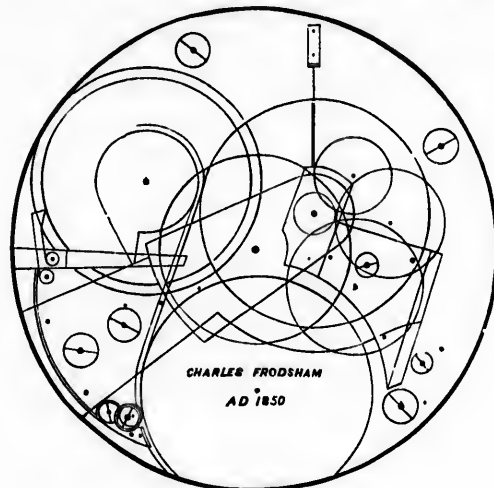
Frodsam's new Calibre for Watches.
