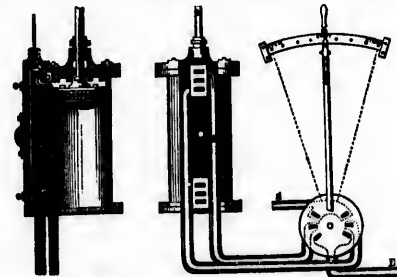
Erskine's Balance Valves, &c., in Section.
