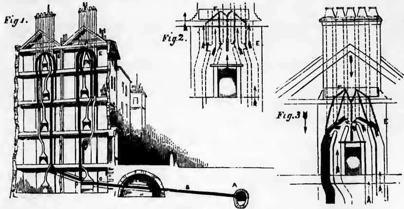
Devey's Smoke Removal Plan.
