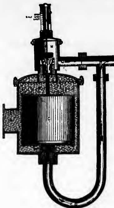
SCALE OF INCHES Mudie's Sallinometer.
