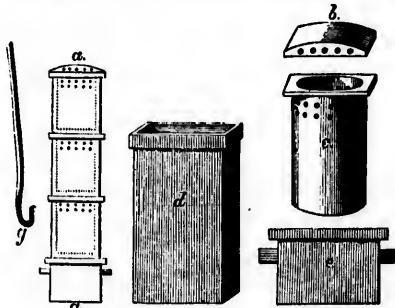
Sadler's Agricultural Chimney Filter Drain.
