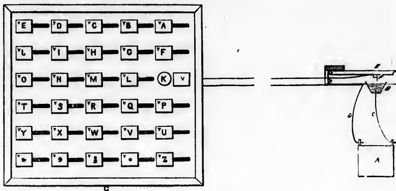
Alexander's Electric Telegraph.
