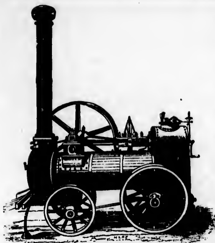
Hornaby's Patent Six-horse Power Portable Steam-engine.
