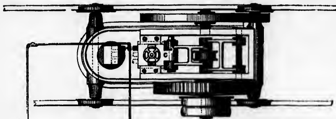
Fairbairn's Patent Riveting Machine. Plan.
