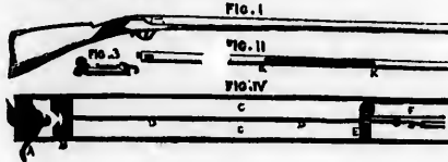
Shaw's India-rubber Air-gun.
