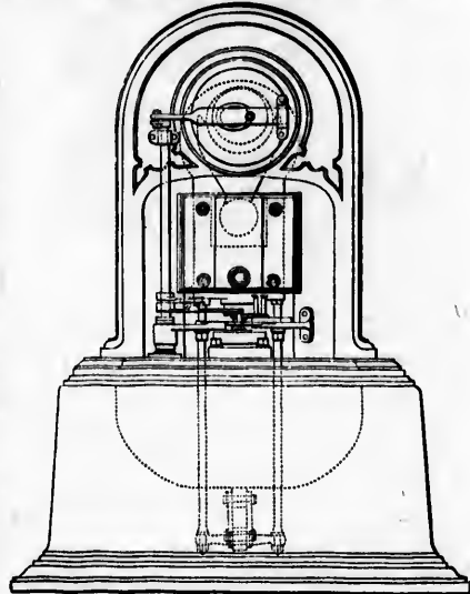
Maudslay & Co.'s Coining Press.
