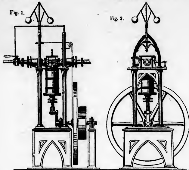
Joyce's Pendulous High-pressure Engine.
