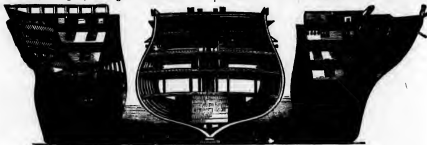
Bow, Stern, and Transverse Sections of H.M.S. "Queen."
