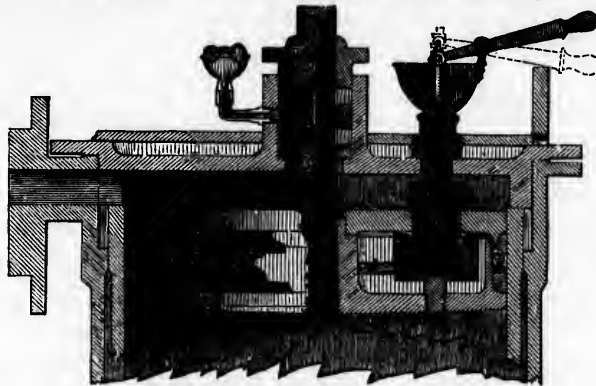
Section showing Hurry's Lubricating Improvements.
