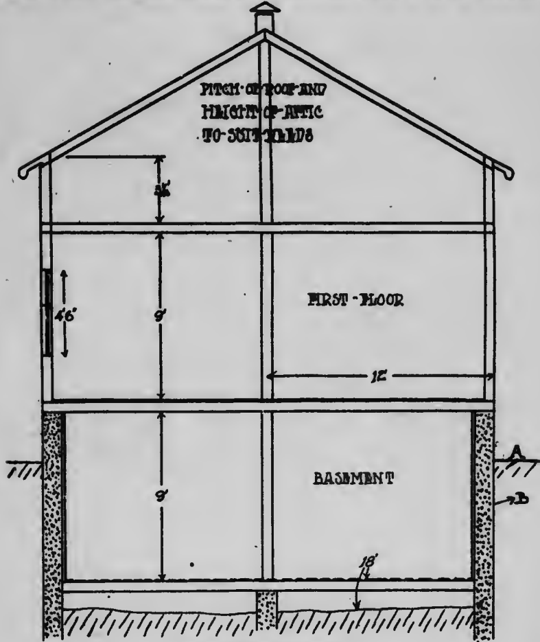
TRANSVERSE SECTION
