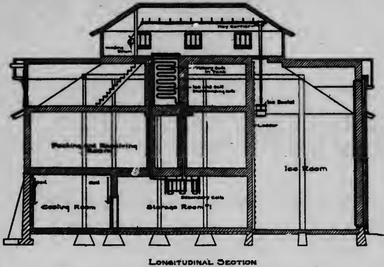
Fig. 2. Diagram showing the arrangement of the farm cold storage of Fig. 1.
