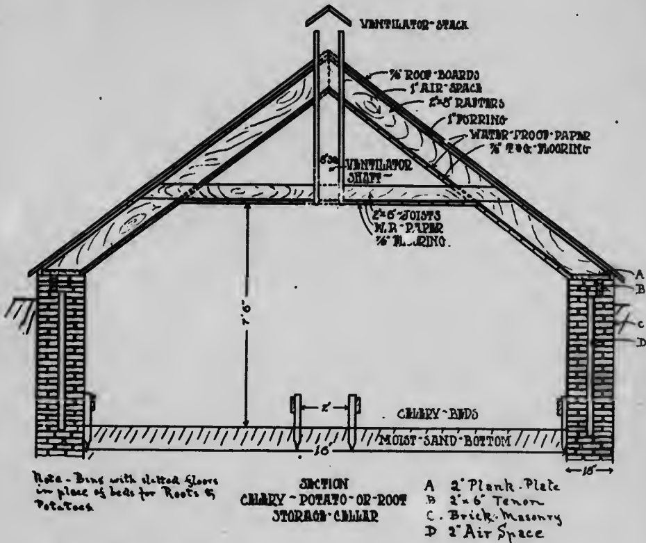
Fig. 13. Diagram showing the section of a celery storage. This building may be adapted to the storage of other vegetables by installing floor and bins.
