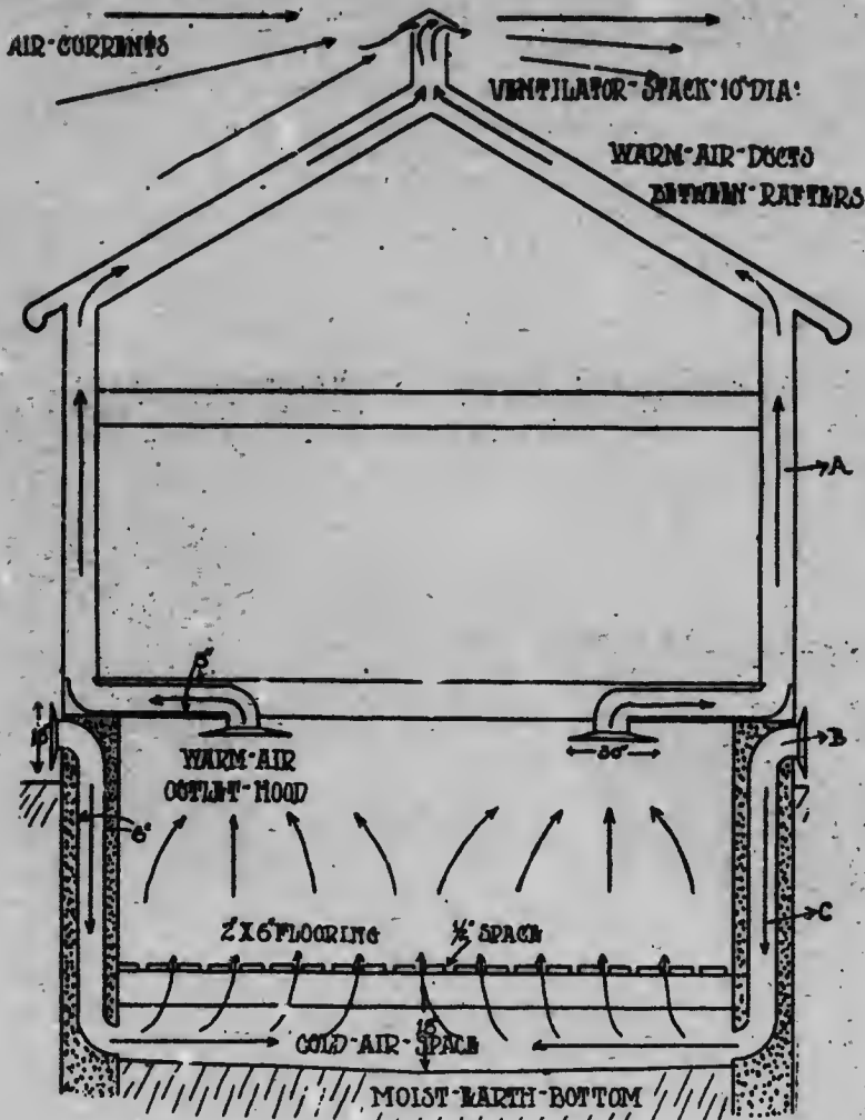
DIAGRAM OF VENTILATING SYSTEM FRUIT-COOL-STORAGE
