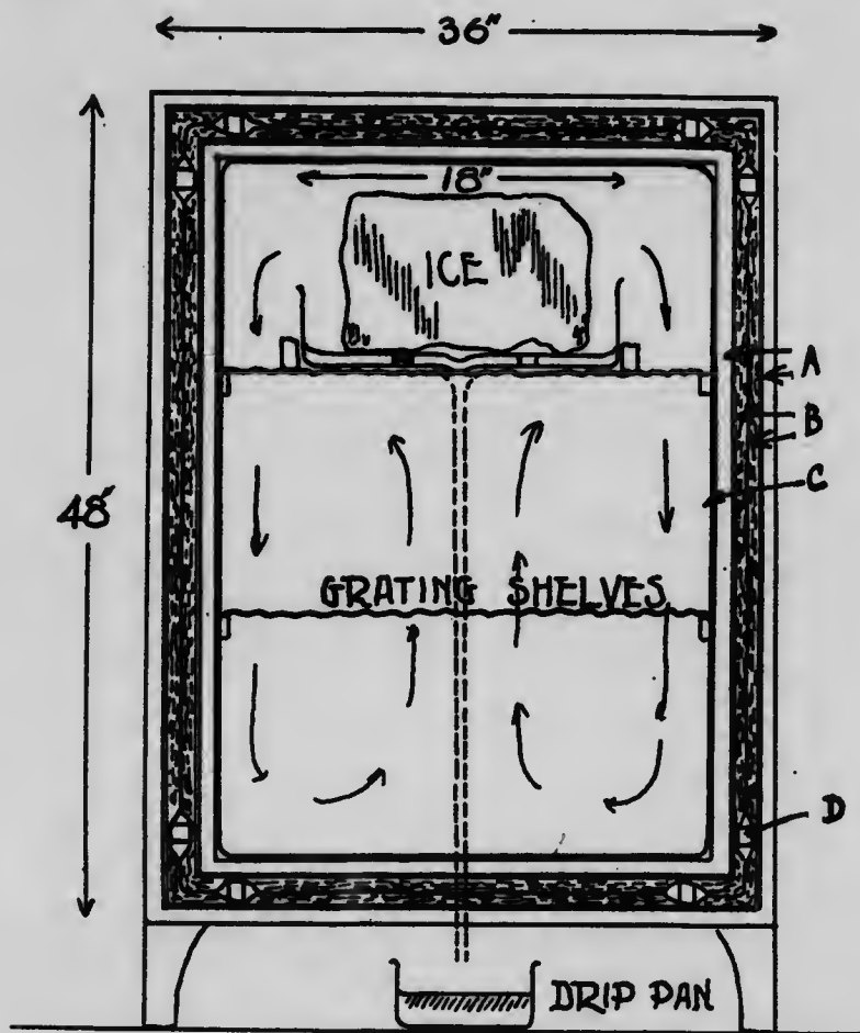
Fig. 3. Diagram of a home-made refrigerator or ice-chest.
