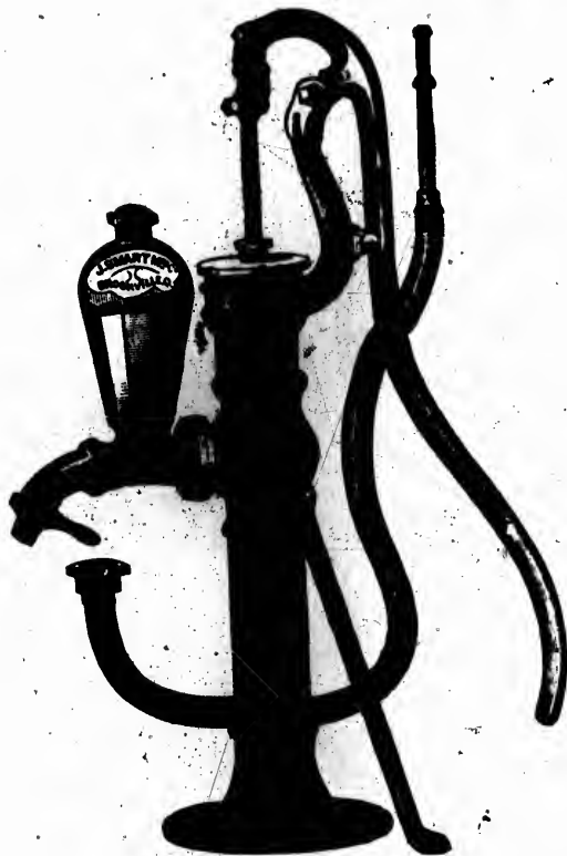
When used for lifting only, unscrew Cap on Air Chamber.
