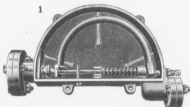
THE HEINTZ STEAM SAVER.
