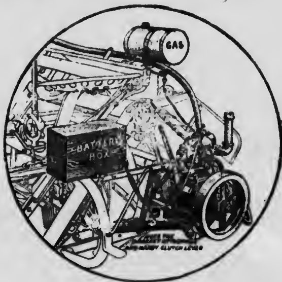
Fig. 2: Small Gasoline Engine used to operate mechanism of Binder while it is being hauled by Horses.
