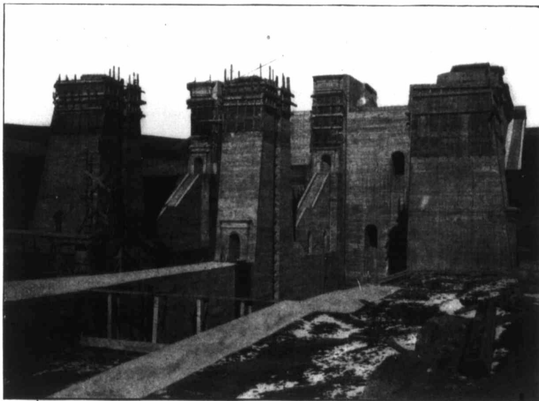
Hydraulic Lift Lock No. 1, Trent Valley Canal, Peterboro, Ont. Richard B. Rogers, Superintending Engineer Built with "Rathbun's Star"
