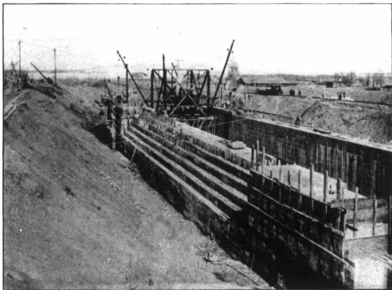
Lock walls in course of construction, Soulanges Canal, with "Rathbun's Star"
