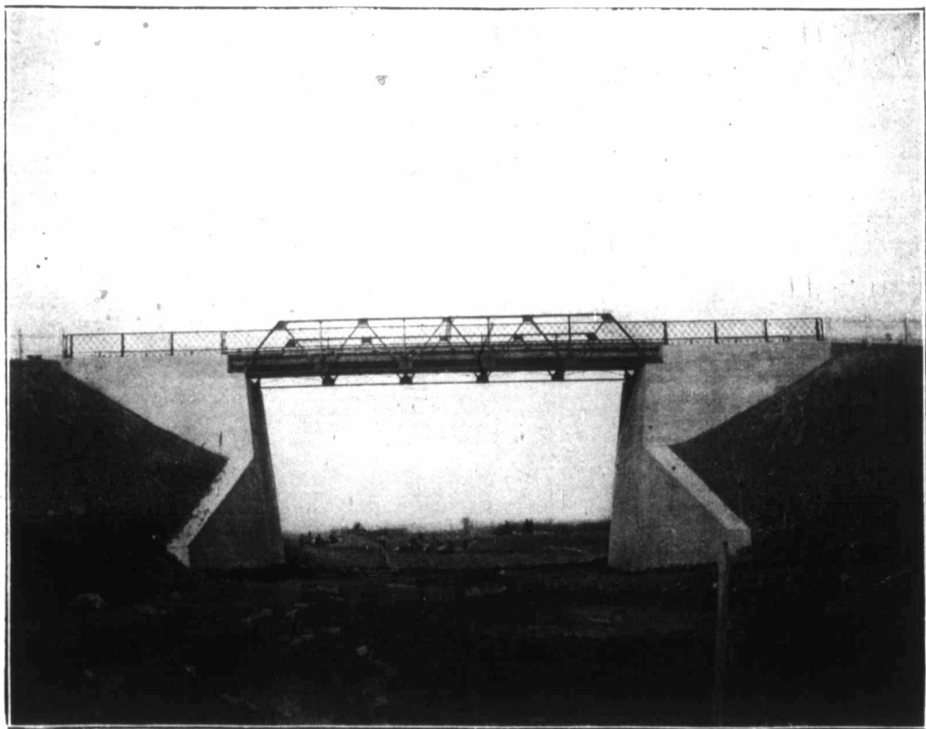
Concrete Bridge Piers (33 feet high), Trent Valley Canal Built with "Rathbun's Star"
