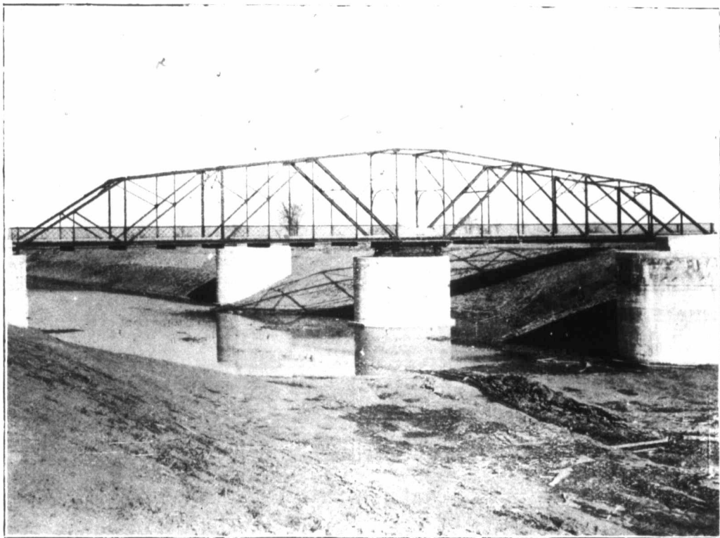
Concrete Bridge Piers, Soulanges Canal Built with "Rathbun's Star"
