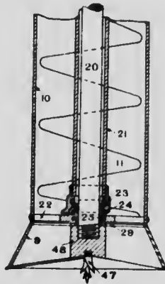
Fig. 49. Vertical section of screw conveyor.
