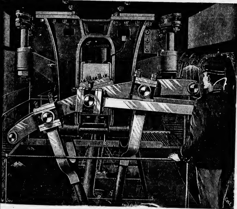
LINK MOTION, MEDIUM CYLINDER. B. — STARBOARD ENGINE-ROOM.
