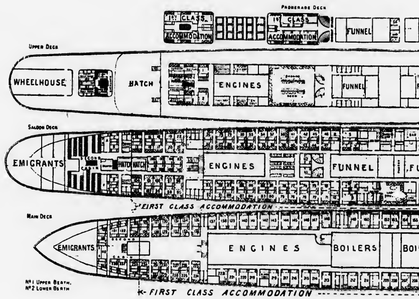
CABIN PLAN OF UMBRIA AND ET
