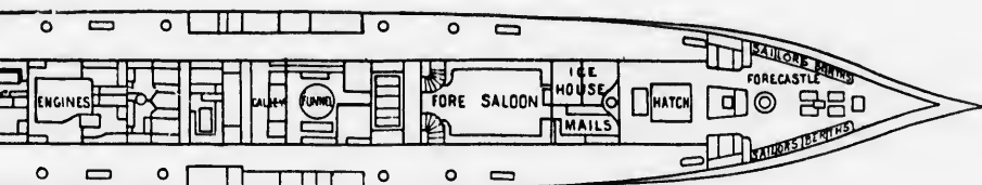
DECK PLAN OF SS. CHINA.
