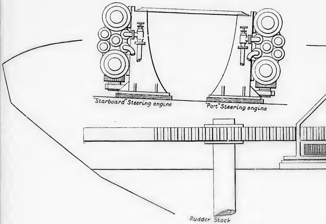
H.—DOUBLE STEAM STEERING GEAR, SS. TEU
