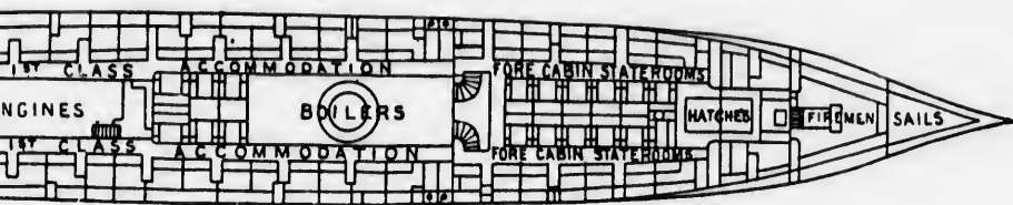
Middle Deck.
