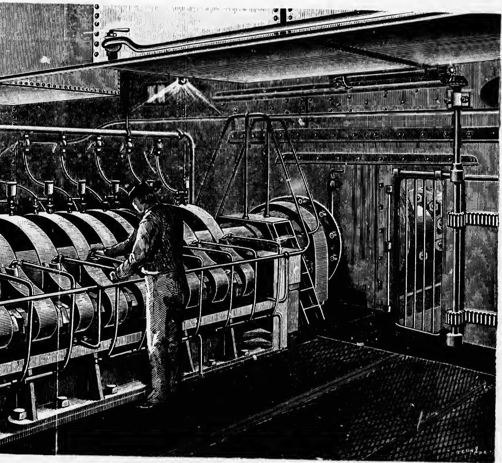
RD THRUST BLOCK, TEUTONIC.
