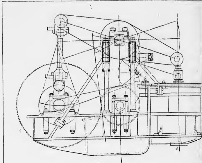
End Elevation, Looking Aft.
