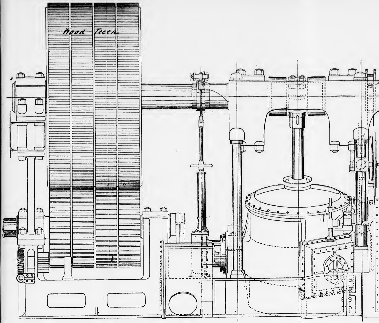
ENGINES OF THE CHINA.
