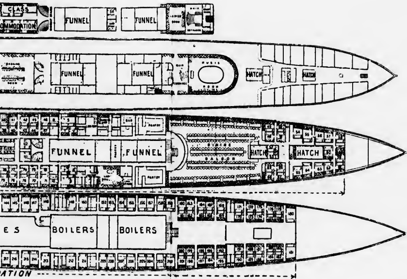
PLAN OF UMBRIA AND ETRURIA.
