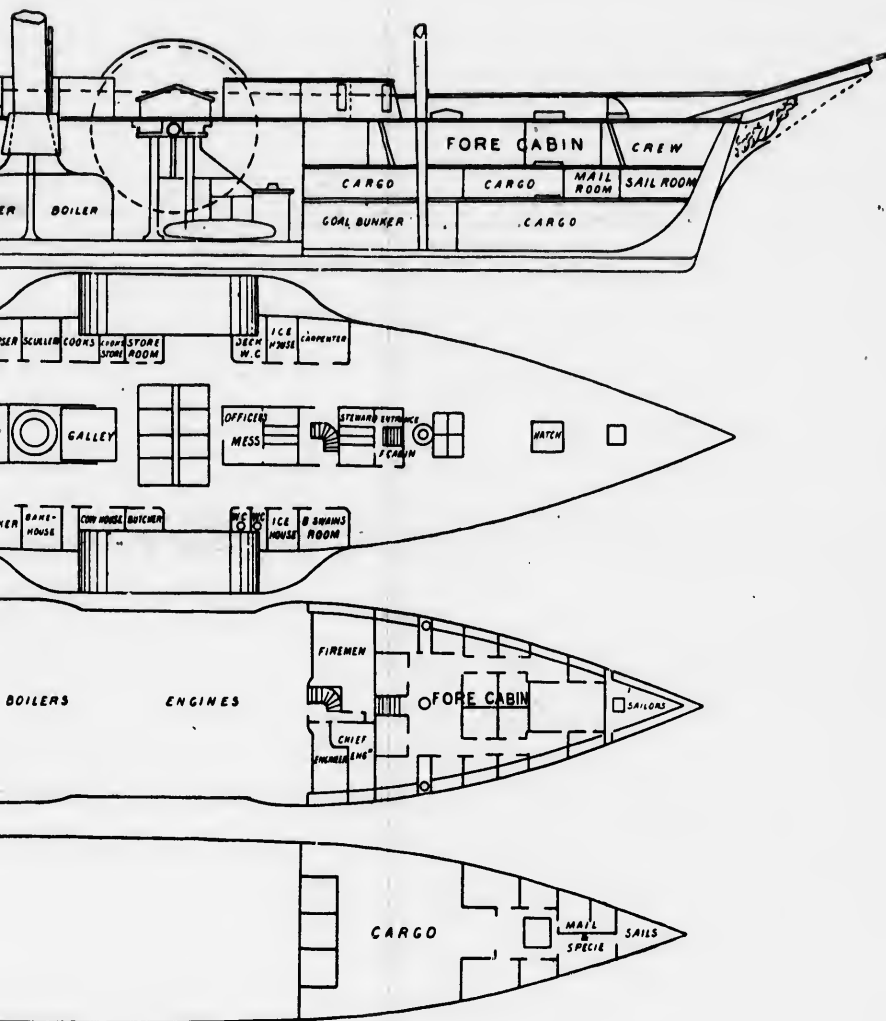
DECK-PLAN OF THE BRITANNIA (CUNARD STEAMER).
