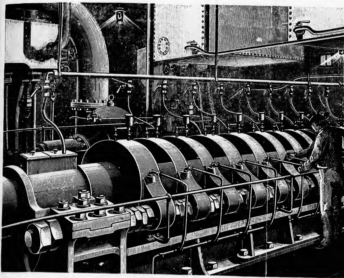
E.—STARBOARD THRUST BLOCK, TEUTONIC.
