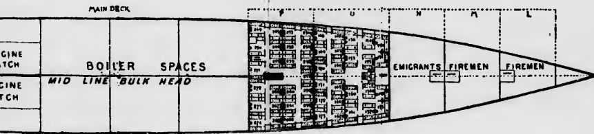
DECK PLAN, CITY OF NEW YORK.
