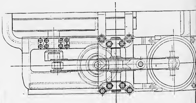
Half Plan.
