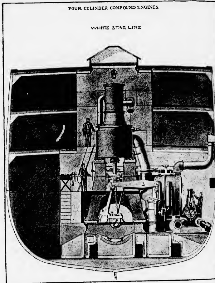
ENGINES OF THE OCEANIC. THWARTSHIP VIEW.
