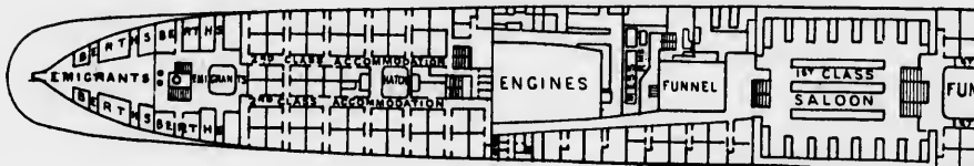
Main Deck.
