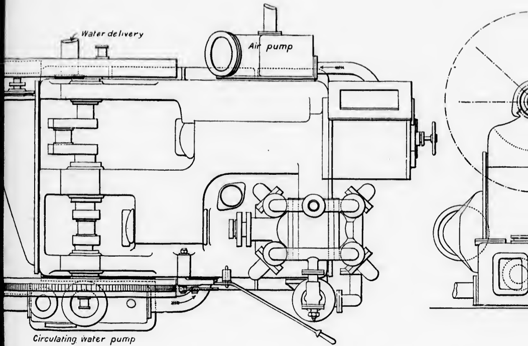
G.—REFRIGERATING CHAMBERS AND GEAR, SS. T
