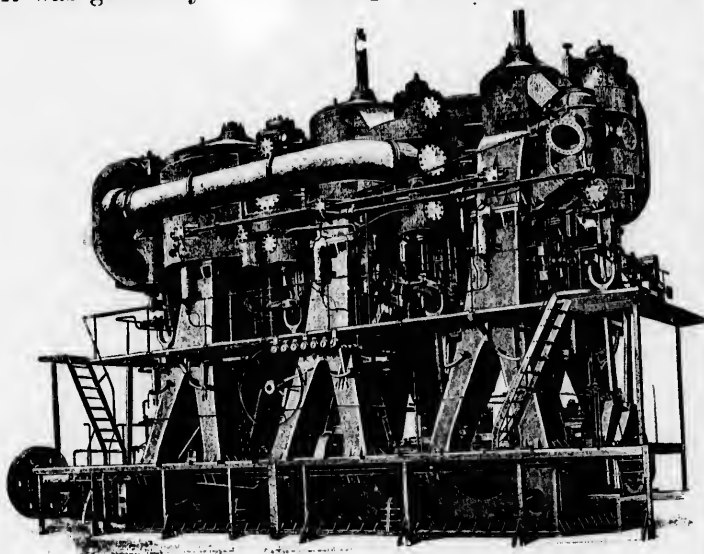
THREE CRANK TRIPLE ENGINES, 1888.
