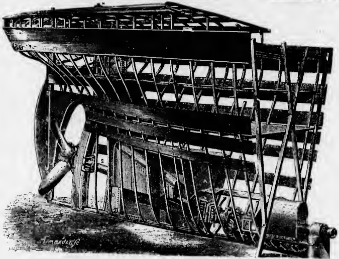
STERN OF BRITANNIC, AS ORIGINALLY FITTED WITH LOWERING PROPELLER, 1874.
