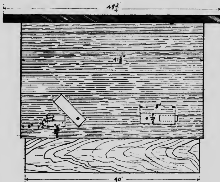
FIG. 2.—End Elevation of 4-Hive Wintering Box, showing arrangement of Entrances.
