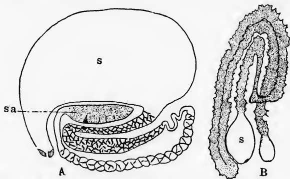
FIG. 172.— A , DIAGRAM OF NEPHRIDIUM (GREEN-GLAND) OF Astacus (after MARCHAL); B , SHELL-GLAND OF Eulimnadia .
