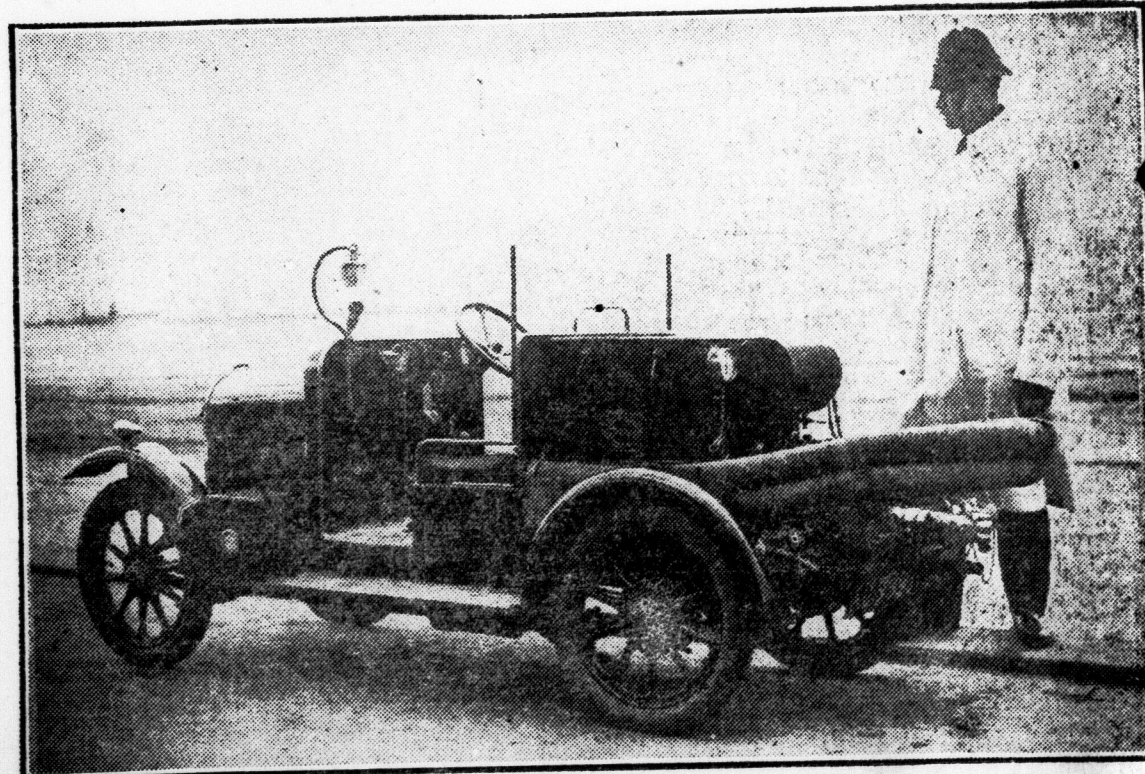
This neat little one-man fire brigade caused quite a sensation on the Blackpool promenade. Compare its size to the police officer. It is a new idea, and is intended for outlying district use
