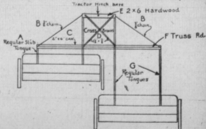
Tractor Hitch for Drawing Two Grain Drills
