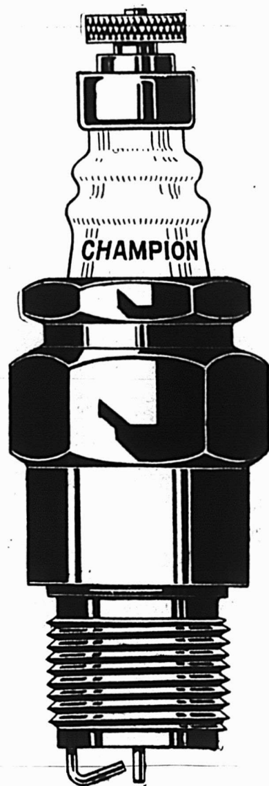
Champion "HEAVY STONE" B-13, ½ pouce B-43, ⅞ pouce, 18. B-53, ⅞ pouce, 18 long. B-73, ¾ pouce. B-83, ¾ pouce long.
