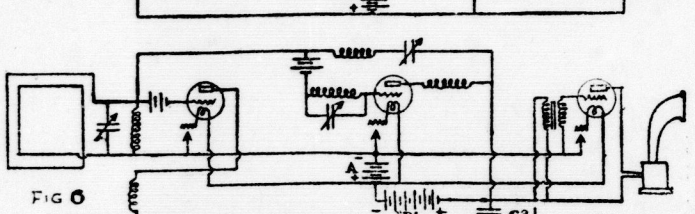
THREE-TUBE SUPER-REGENERATIVE CIRCUITS.
