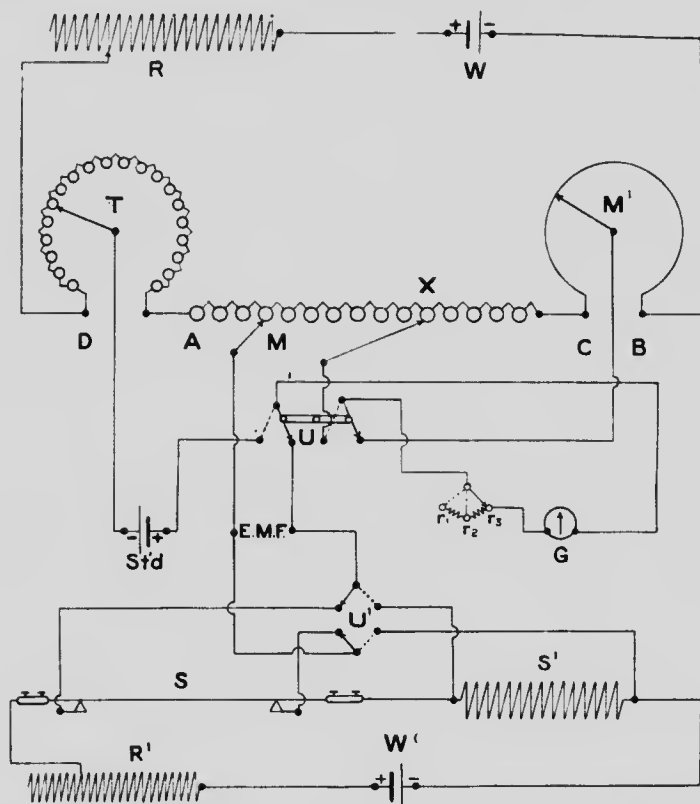
Fig. 7. Arrangement of circuits for electrical resistance measurements.
