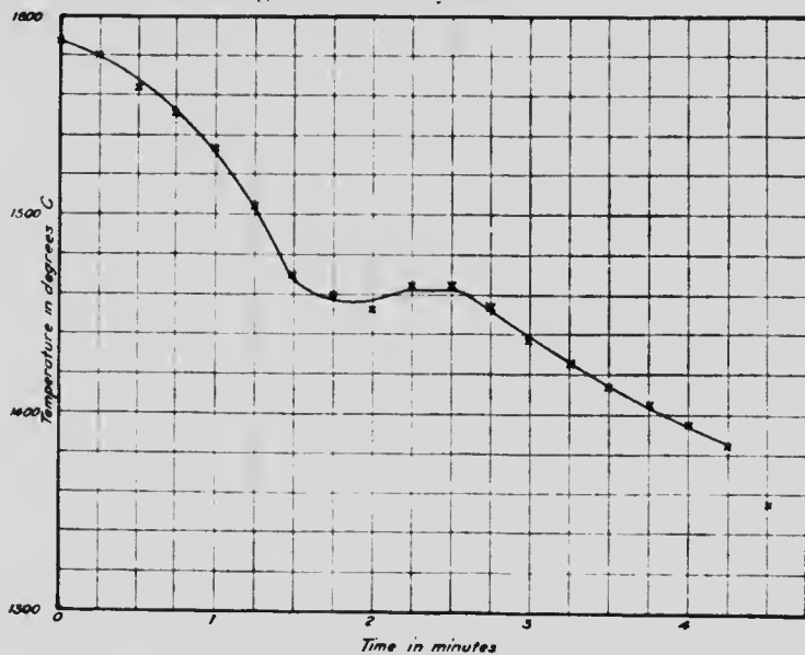
Fig. 2. Cooling curve—melting point—cobalt.
