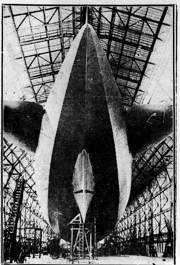
A remarkable picture of the ZR-3, showing its structural resemblance to a fish. This, taken from the stern, shows the tail fins and rudder. The bulk of the zeppelin, as large as an ocean liner, may be gauged from the ladders.
