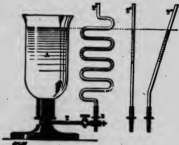
Fig. 165. — Vases communicants.
