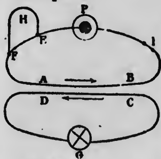
Fig. 213.—Induction.
