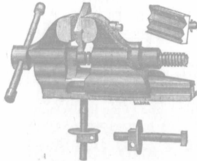
PIPE-EXTRA JAW.
