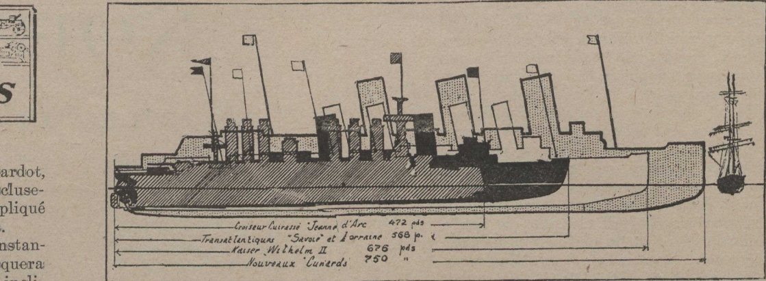
Silhouettes comparatives: la "Jeanne d'Arc," la "Lorraine," le "Kaiser Wilhelm der Grosse" et les nouveaux Cunards.
