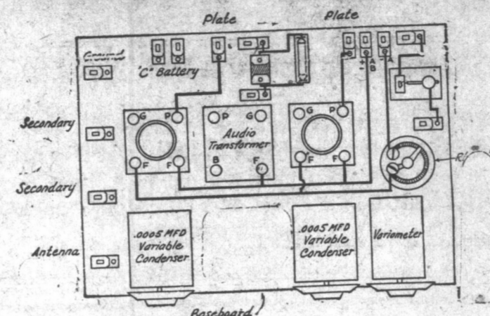
A Convenient Test Board
