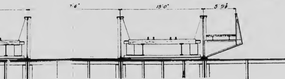
FLOOR AS BUILT
