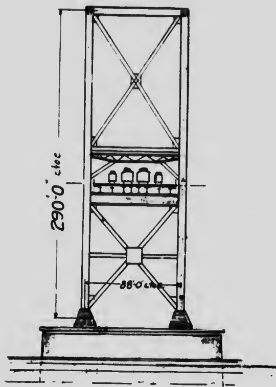
- DESIGN "D" - - Cross Section of Main Pier. -
