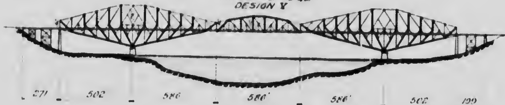
FIG 3 S' LAWRENCE BRIDGE CO LTD QUEBEC BRIDGE DESIGN A-B-X
