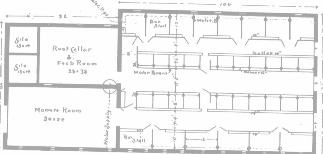
GROUND PLAN - BASEMENT BARN OF H. CARGILL & SON, CARGILL, ONT. Size of Basement Walls 72 x 156 feet. Concrete floors put in this building with Thorold Cement.
