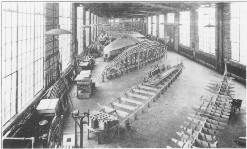
FLYING BOAT HULL CONSTRUCTION—CANADIAN AEROPLANES LIMITED.
