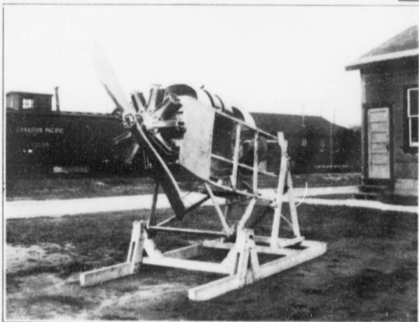
CLERGET ENGINE ON ROCKING NACELLE.
