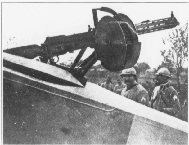
GERMAN PARABELLUM MOUNTING.
