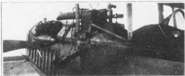
SHOOTING THROUGH PROPELLER. ✓
