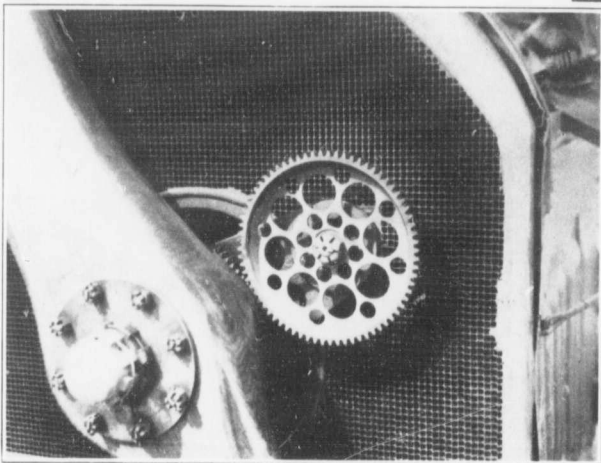
SYNCHRONIZING GEAR. ✓
