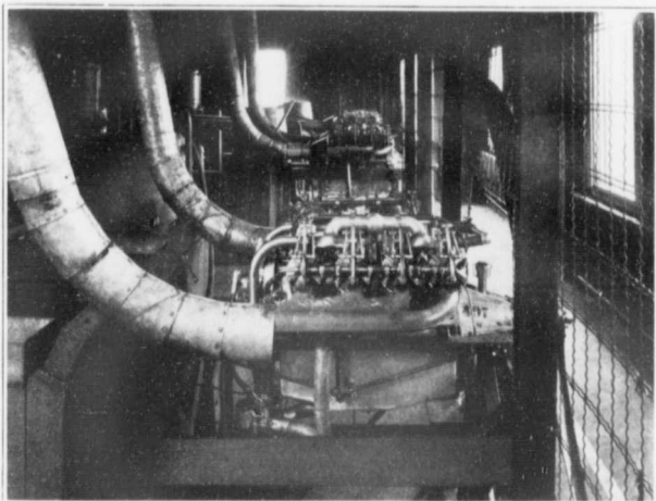
ENGINES MOUNTED FOR TEST.
