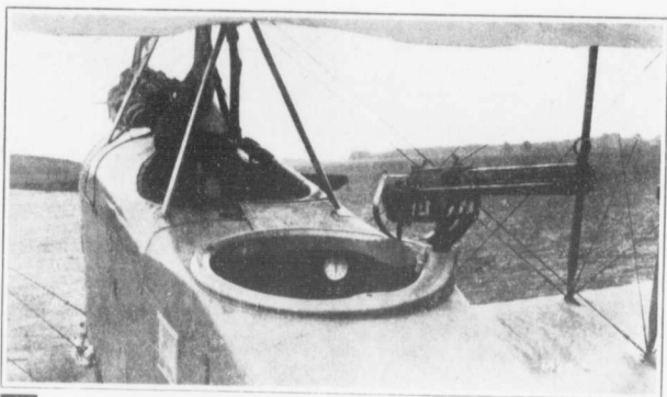
OBSERVERS' GUN MOUNTING
