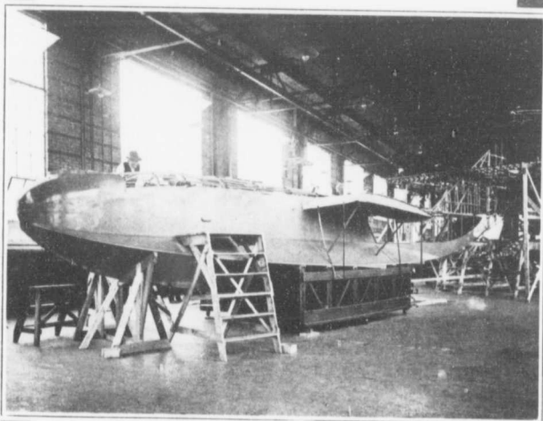
FLYING BOAT HULL UNDER CONSTRUCTION.
