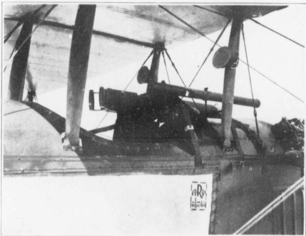
SYNCHRONIZED VICKERS' GUN. ✓
