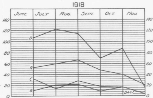
RAF CAN - CRASH COMPARISON SHOWING EFFECT OF INTRODUCTION OF THE ARMOUR HEIGHTS SYSTEM
