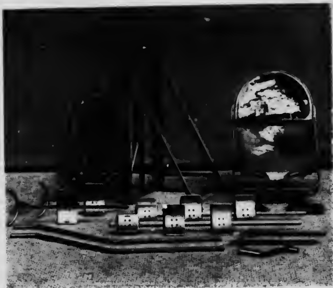
FIG. 12.—AUTHOR'S TRANSPORTABLE OPERATION-TABLE. Showing the various segments and the mountings of the legs. Detached pieces shown.
