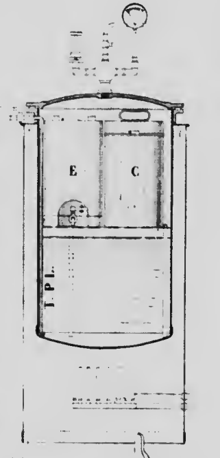
FIG. 26.—DIAGRAMMATIC SECTION OF VAPOUR STOVE.
