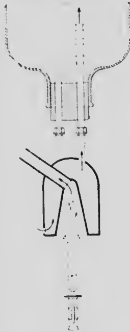
FIG. 34. THERMO-SIPHON FOR HEATING STERILE SOLUTIONS.
