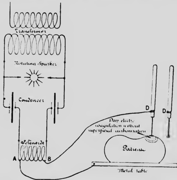
FIG. 605.—ELECTRO-COAGULATION WITHOUT SUPERFICIAL CARBONIZATION (AUSTIN'S MOST RECENT APPARATUS). (DIAGRAMMATIC.)
