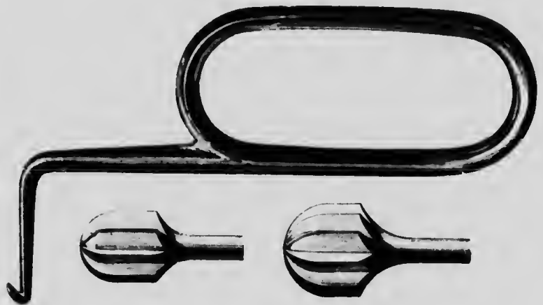
FIGS. 850, 851, AND 852. CROCHET FOR THE WALL OF THE TYMPANUM; CYLINDRO-SPHERICAL BURRS OF 16 AND 20 MILLIMETRES RESPECTIVELY.
