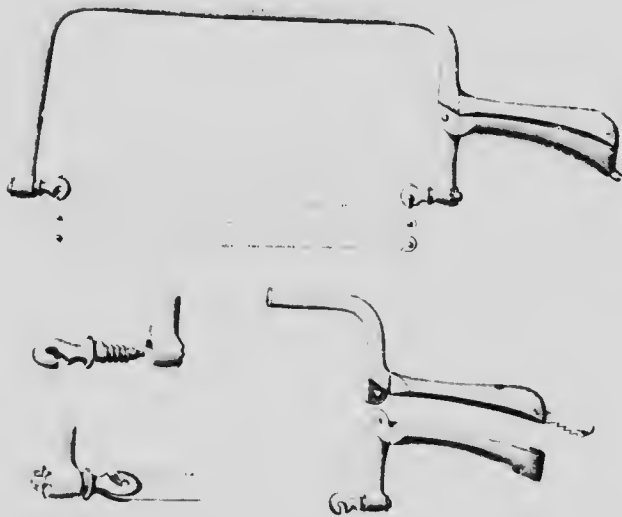
FIG. 386. SAW WITH RETRACTING BLADE, WITH VARIABLE TENSION.
