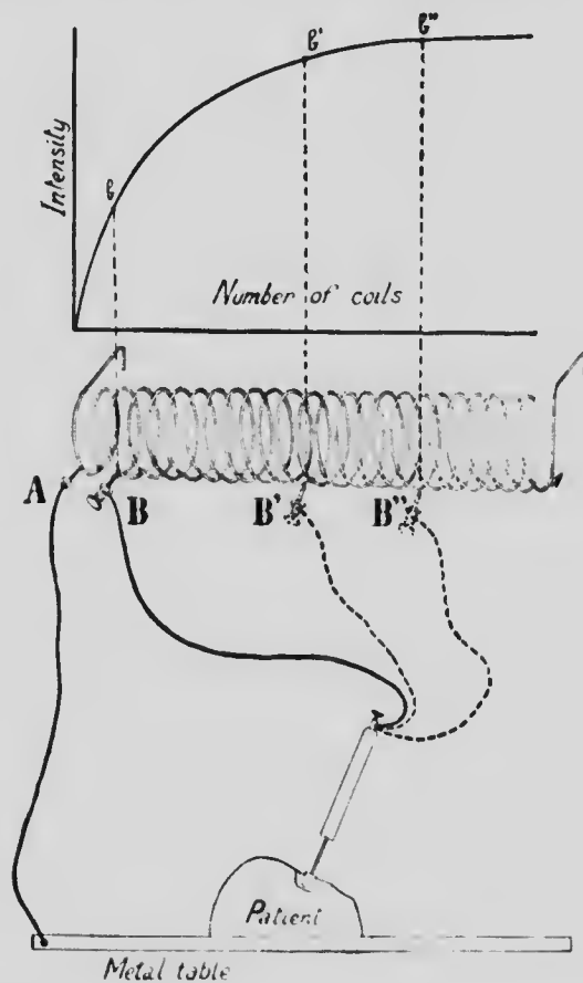
FIG. 607. DIAGRAMMATIC SCHEME INDICATING THE VARIATION OF INTENSITY OF CURRENT WHICH FOLLOWS INTRODUCTION OF A GREATER OR LESS NUMBER OF SPIRAL COILS INTO THE CIRCUIT.
