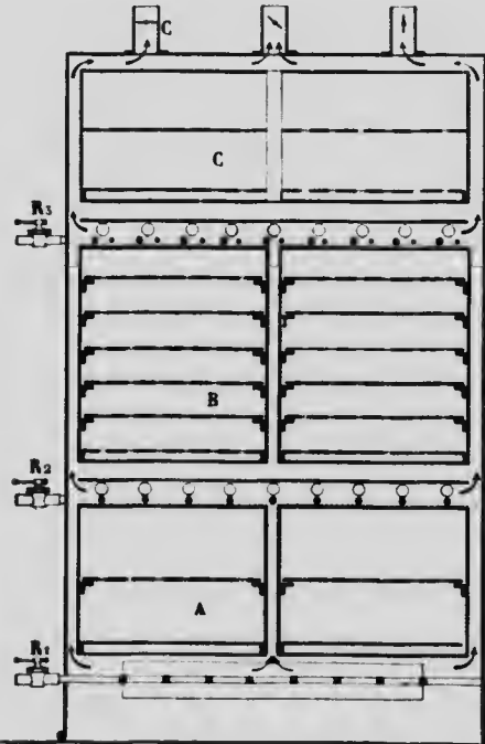
FIG. 25.—DIAGRAMMATIC SECTION OF AUTHOR'S LARGE STOVE.
