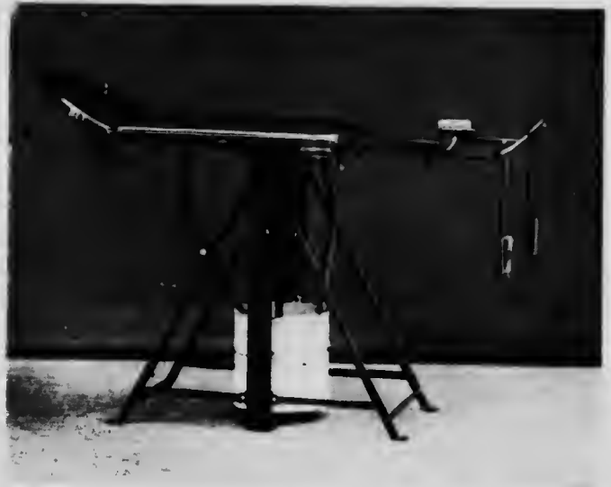
FIG. 13. —ARTHUR'S TRANSPORTABLE OPERATION-TABLE. Horizontal position, and rectangular arrangement of leg-supports.
