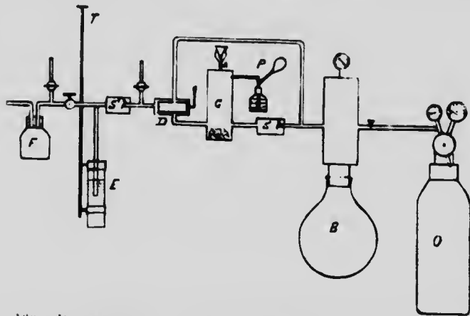
FIG. 160. DIAGRAMMATIC SKETCH OF DOYEN'S APPARATUS FOR THORACIC HYPERPRESSURE.
