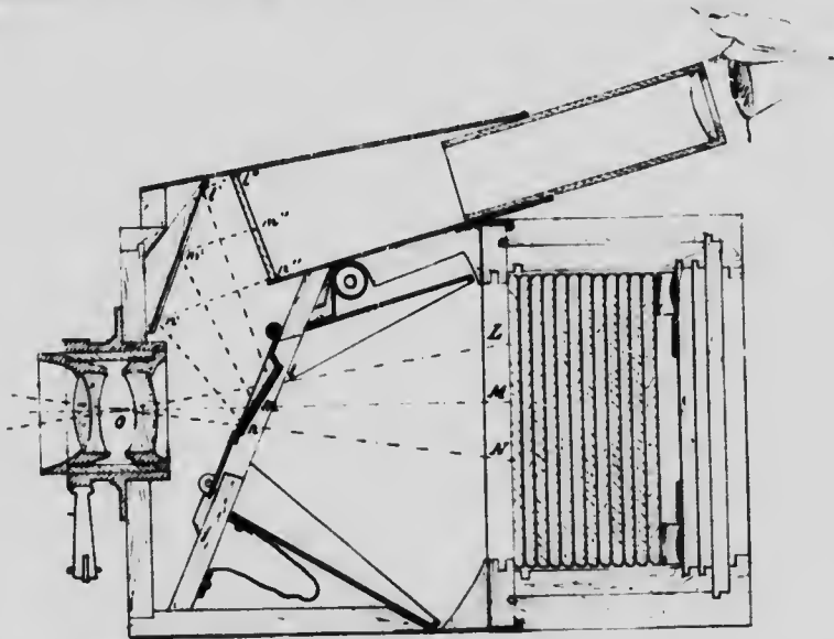
FIG. 35. SECTION OF DUPED'S PHOTOGRAPHIC APPARATUS.
