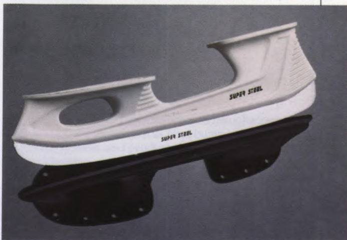
The ICM Pro Super Steel has an integrated runner and holder system.
