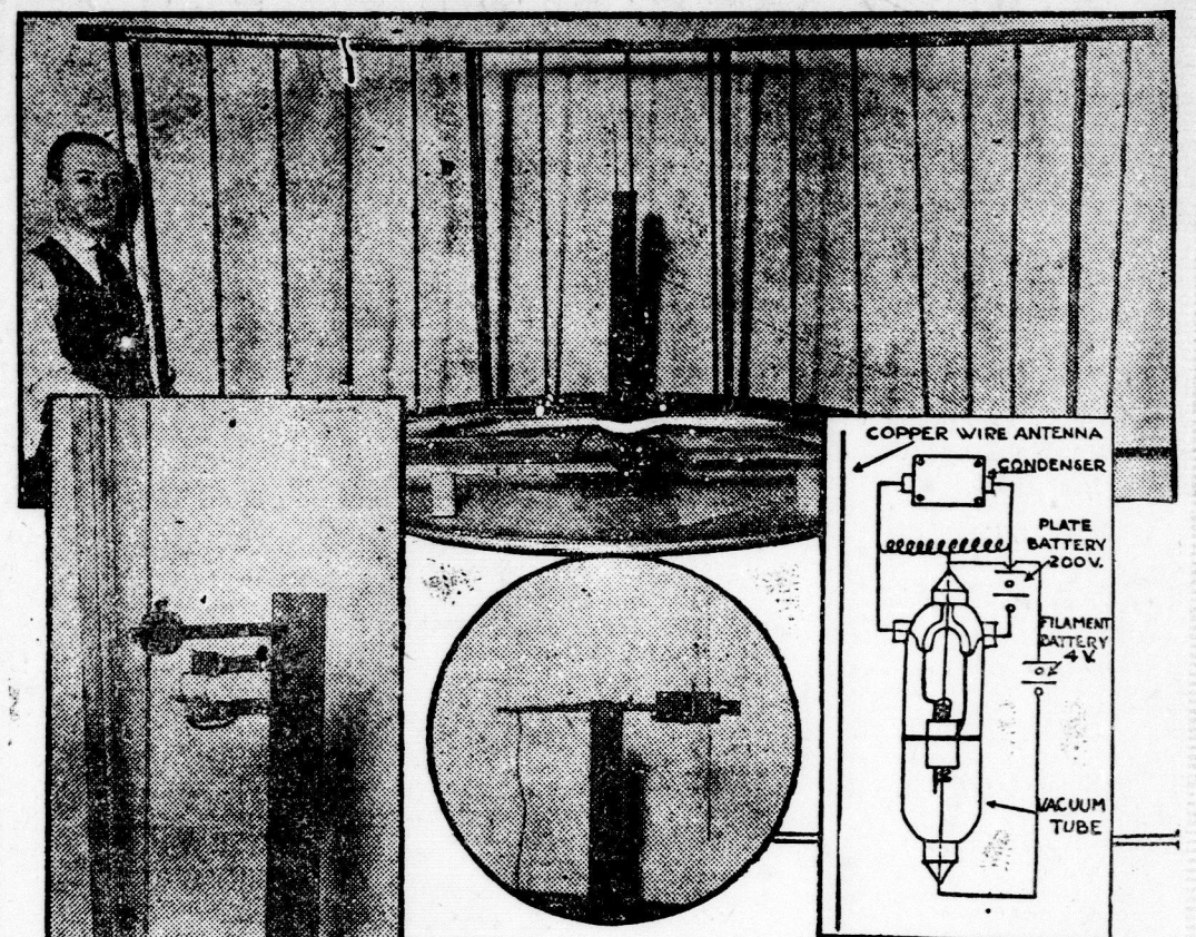
MARCONI'S "RADIO SEARCHLIGHT" ABOVE. BELOW, LEFT, CLOSE-UP OF THE TRANSMITTER; CENTER, THE RECEIVER; RIGHT, DIAGRAM OF THE TRANSMITTER.
