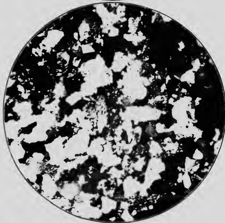
Fig. 1. Feldspathic Quartzite near Otter Lake A 28.
