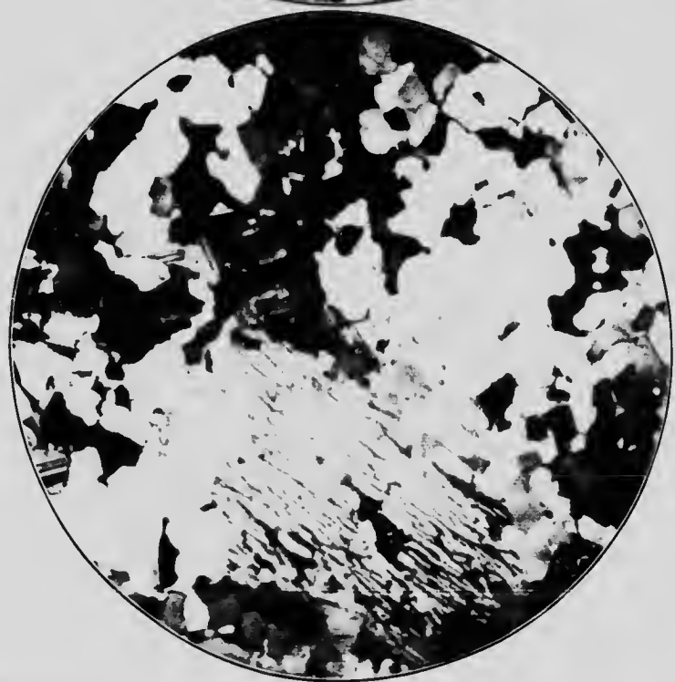
Fig. 1. Granite associated with Gneiss from Slungwak Lake, V. 25.
