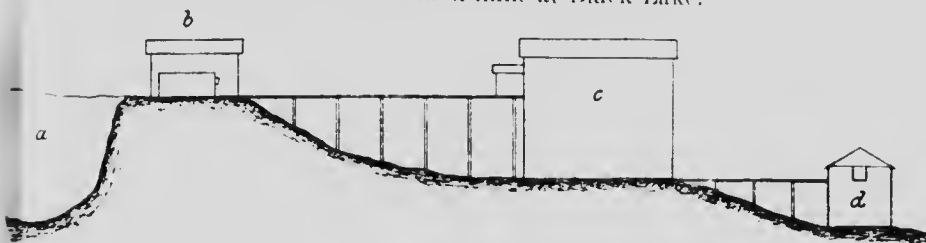
FIG. 30 - Type of a sloping mill.
