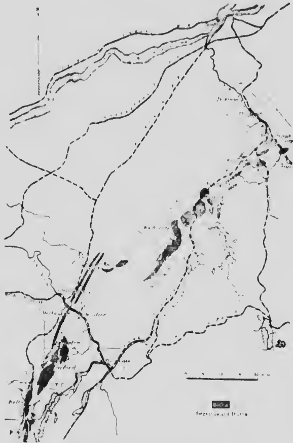
FIG. 2—Map Showing the distribution of Serpentine in the Eastern Townships of Quebec. By Fritz Cirkel, M.E.
