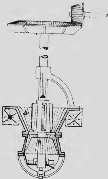
FIG. 18. Rotary Crusher as manufactured by Butterworth & Lowe, Grand Rapids, Mich.
