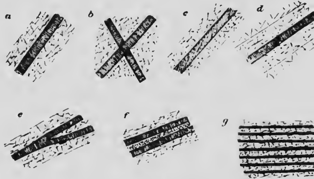
FIG. 4—Typical Asbestos Beds.
